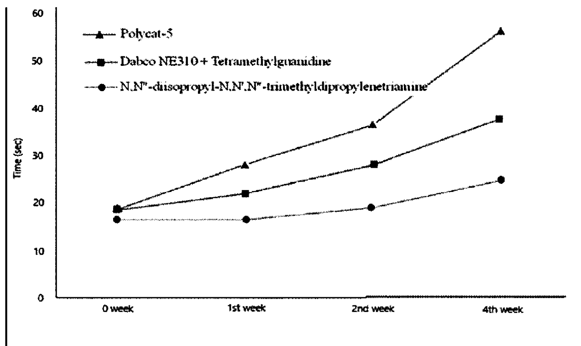
Figure 4: Time in seconds to 80% Maximum Height at 0 week, 1 week, 2 weeks and 4 weeks
