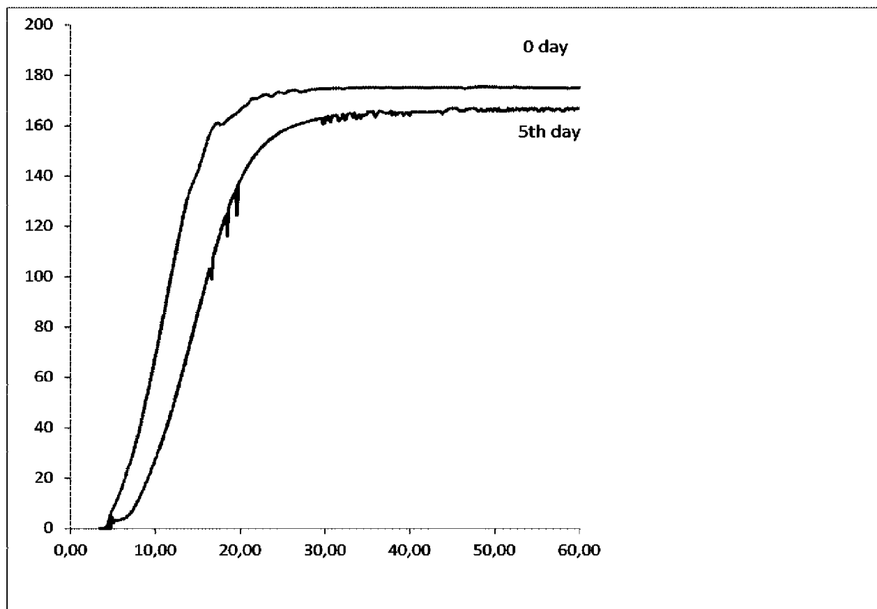
Figure 13: Rate of Rise profiles for foam made in accordance with Example 16 at 0 days and 5 days
