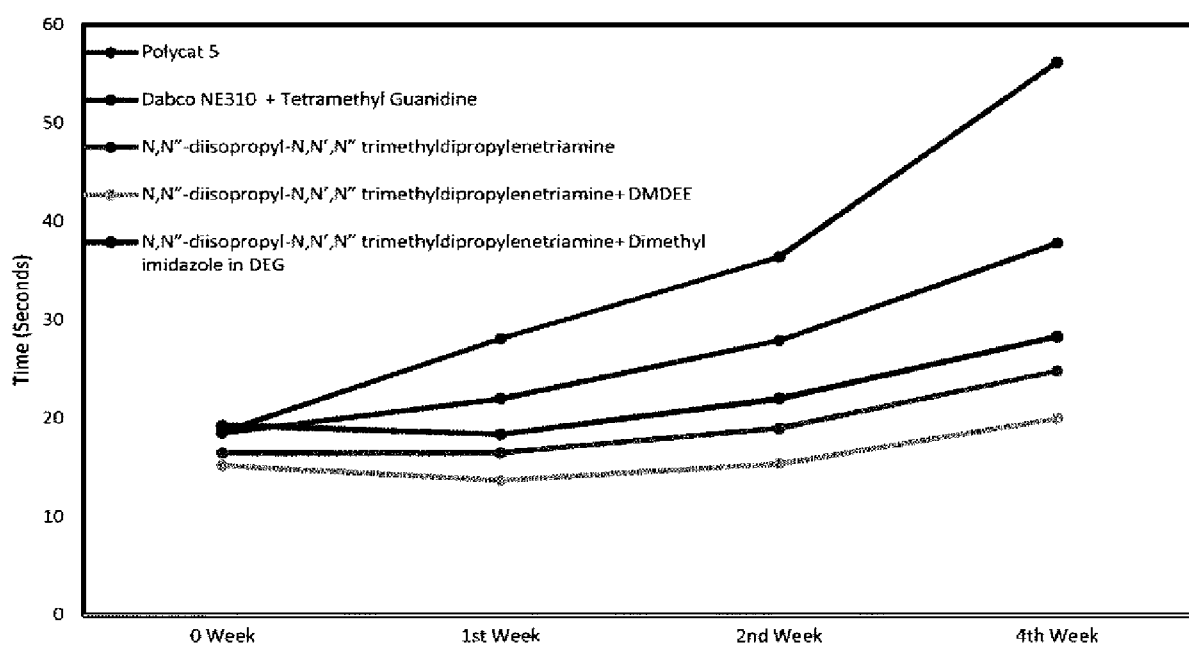
Figure 16: Time in seconds to 80% Maximum Height at 0 week, 1 week, 2 weeks and 4 weeks
