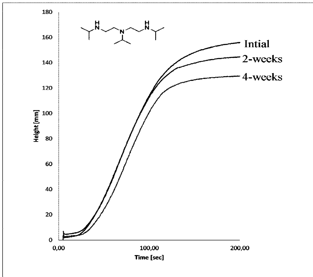
Figure 7: Rate of Rise profiles for foam made in accordance with Example 3 at 0 week, 2 weeks and 4 weeks
