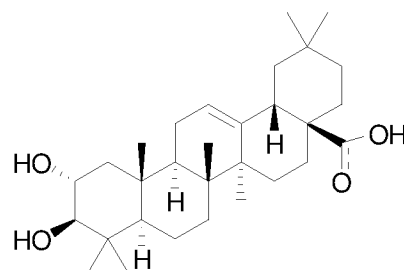
Maslinic acid
