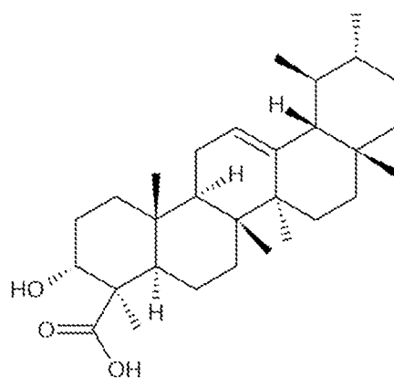
β-boswellic acid
