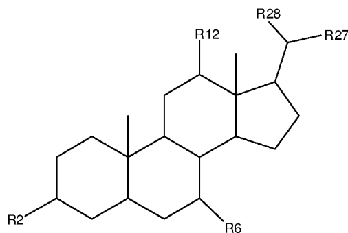
Formula 4,
