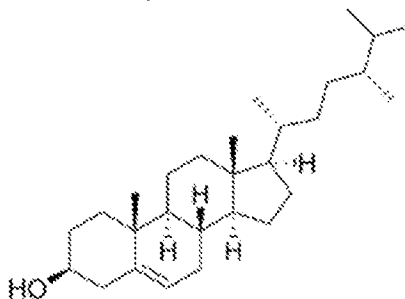
Campesterol
