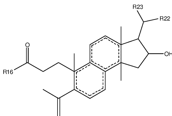
Formula 2,
