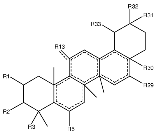
Formula 6,
