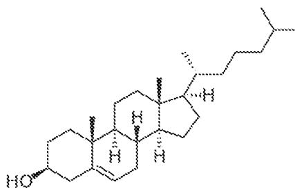
Cholesterol
