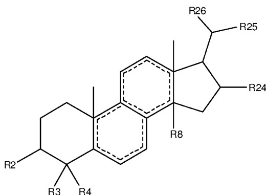
Formula 3,
