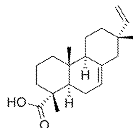
Isopimaric acid
