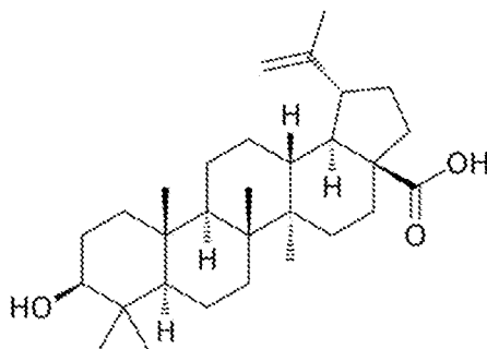
Betulinic acid
