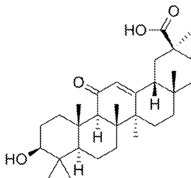
Glycyrrhetic acid
