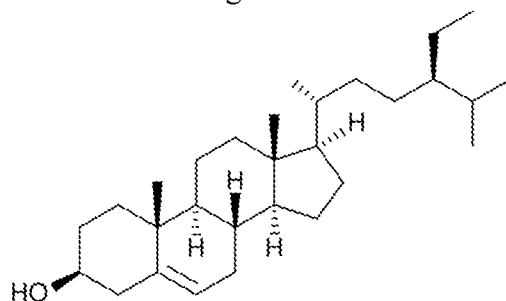
\beta -sitosterol
