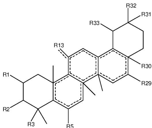
Formula 6,
