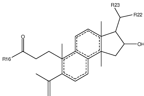
Formula 2,
