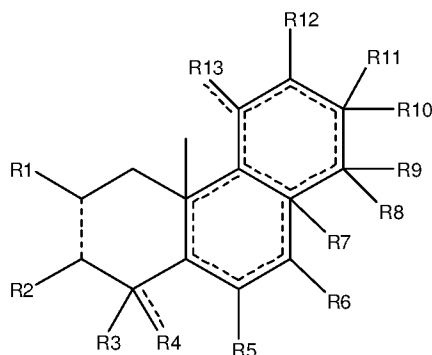
Formula 1,
