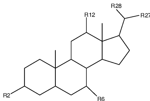
Formula 4,
