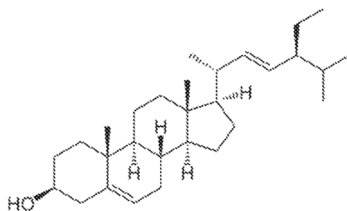
Stigmasterol
