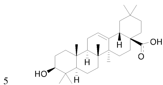
Oleanolic acid
