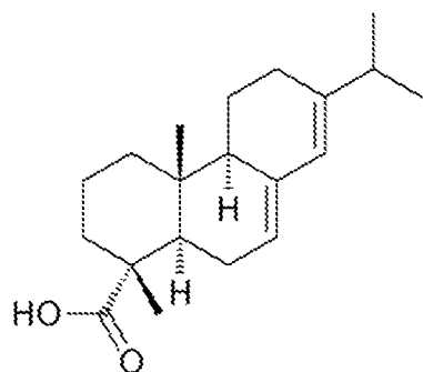
Abietic acid
