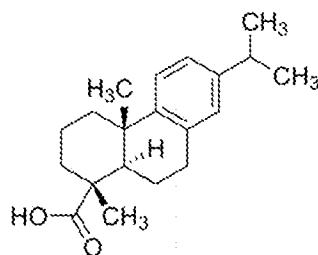
Dehydroabietic acid
