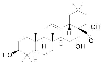
Echinocystic acid
