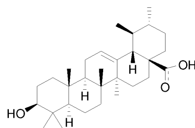
Ursolic acid
