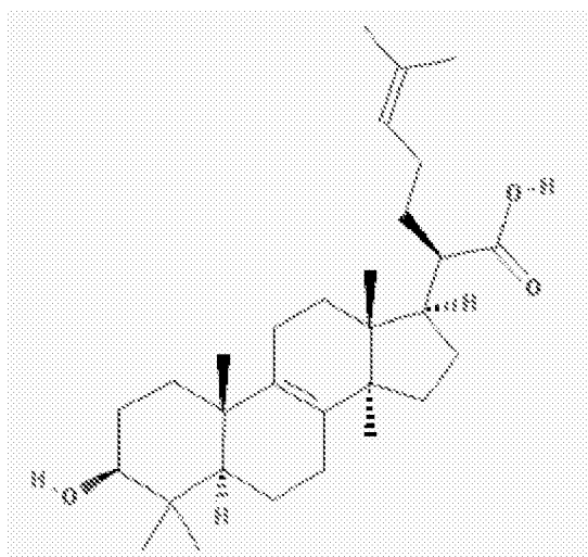
Trametenolic acid
