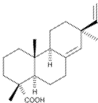
Pimaric acid
