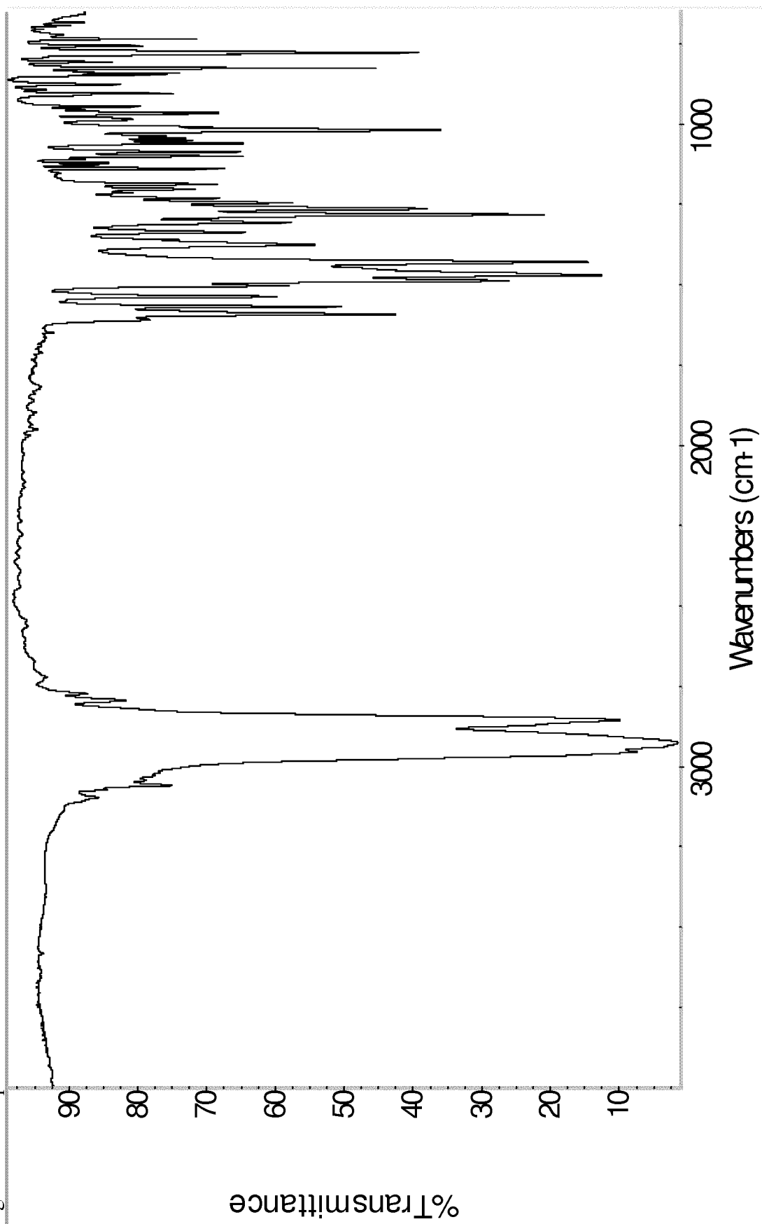
Figure 17: IR spectrum of form F
