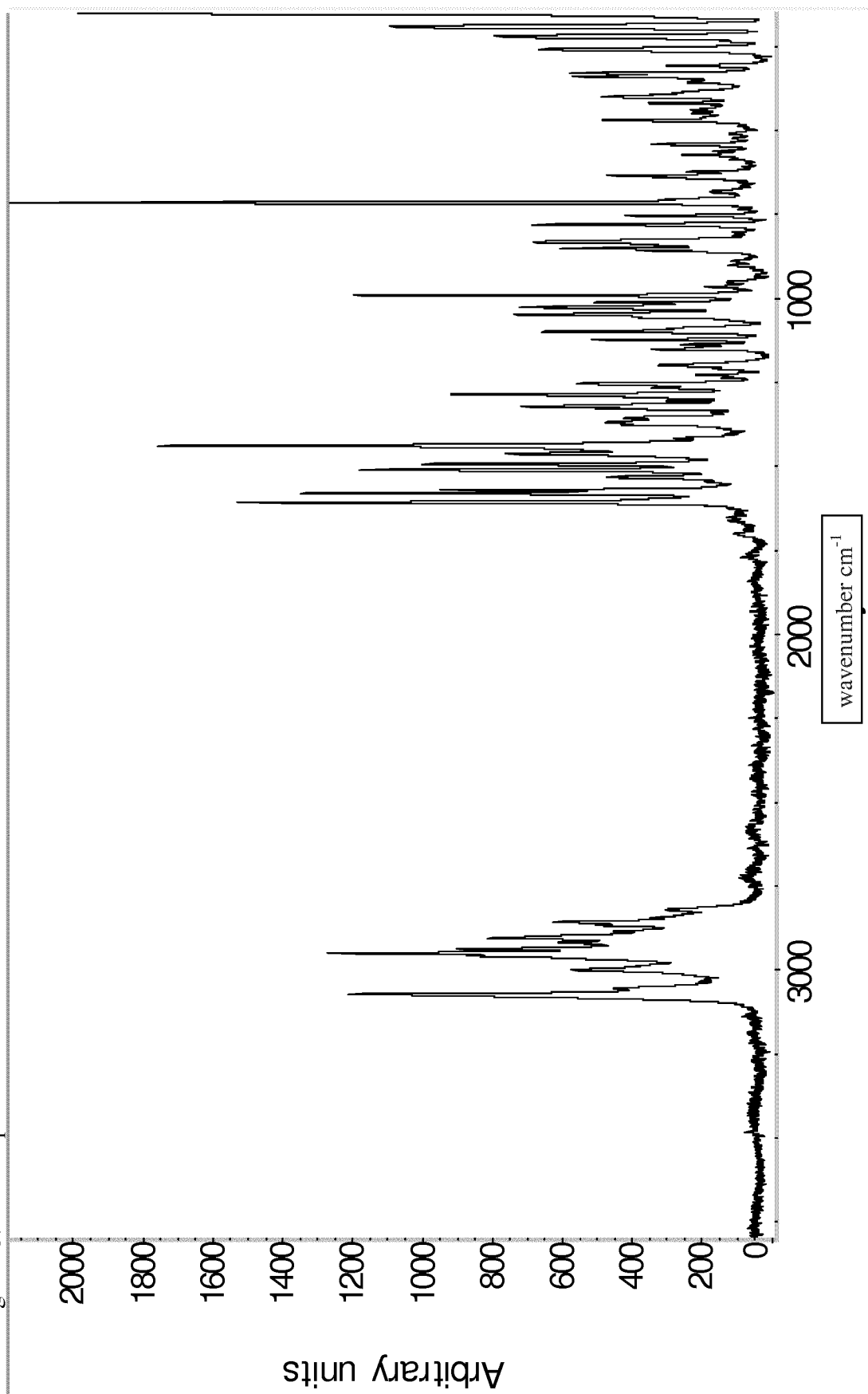
Figure 23: Raman spectrum of form H
