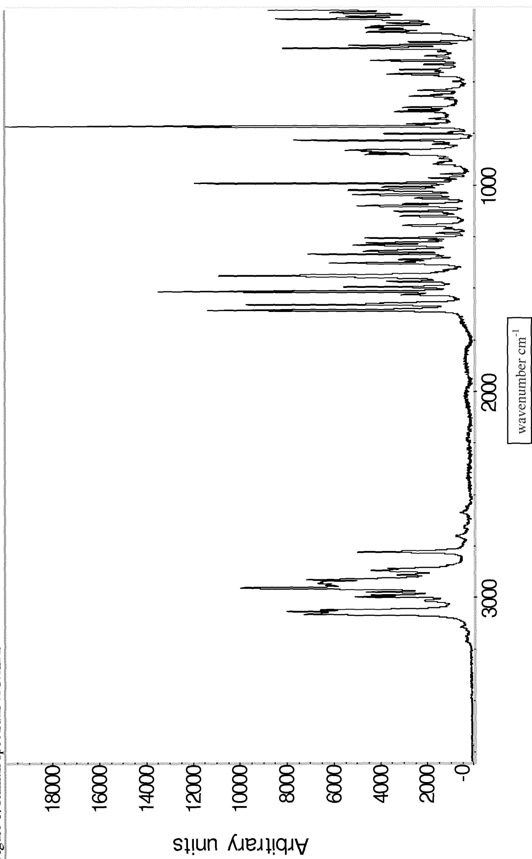
Figure 6: Raman spectrum of form B
