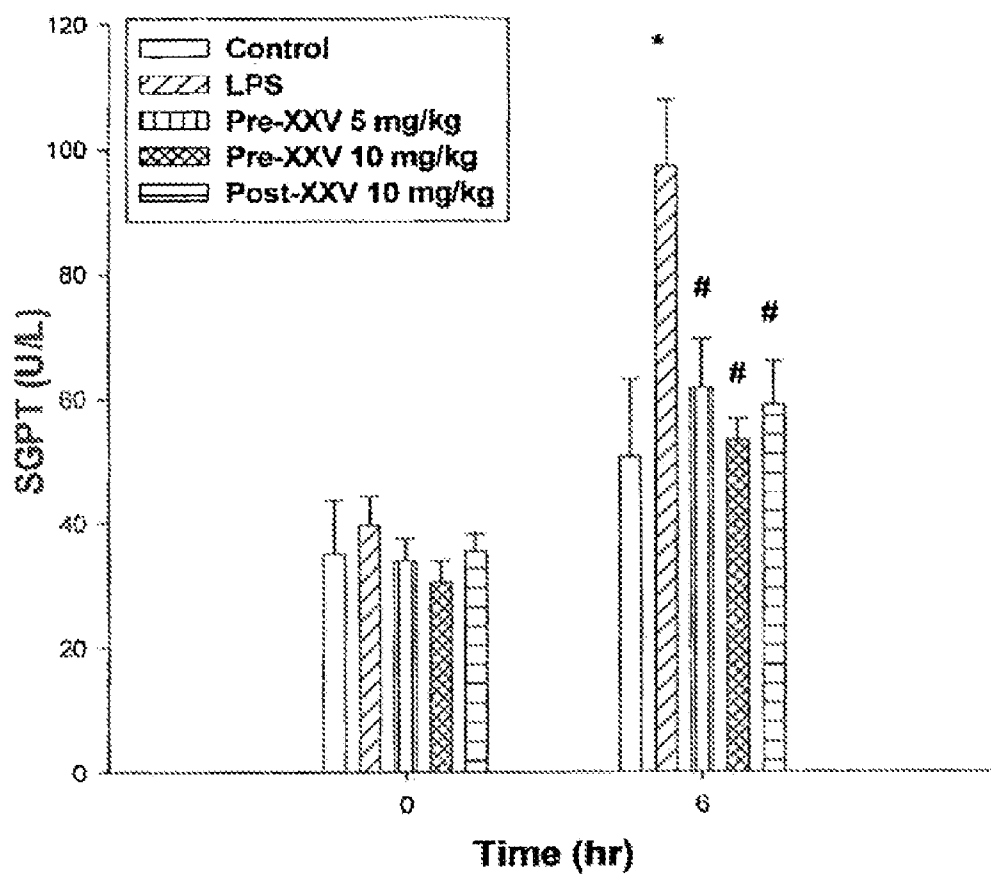
Figure 4. Effects of pre-treatment with XXV (5 mg/kg, i.v., n=9 and 10 mg/kg, i.v., n=10) and post-treatment XXV (10 mg/kg, i.v., n=6) on SGPT at 0 and 6 hr after LPS-treated rat (n=10). Data represent mean \pm S.E.M., * p < 0.05 : LPS vs. Control (n=4) and # p < 0.05 : XXV vs. LPS.
