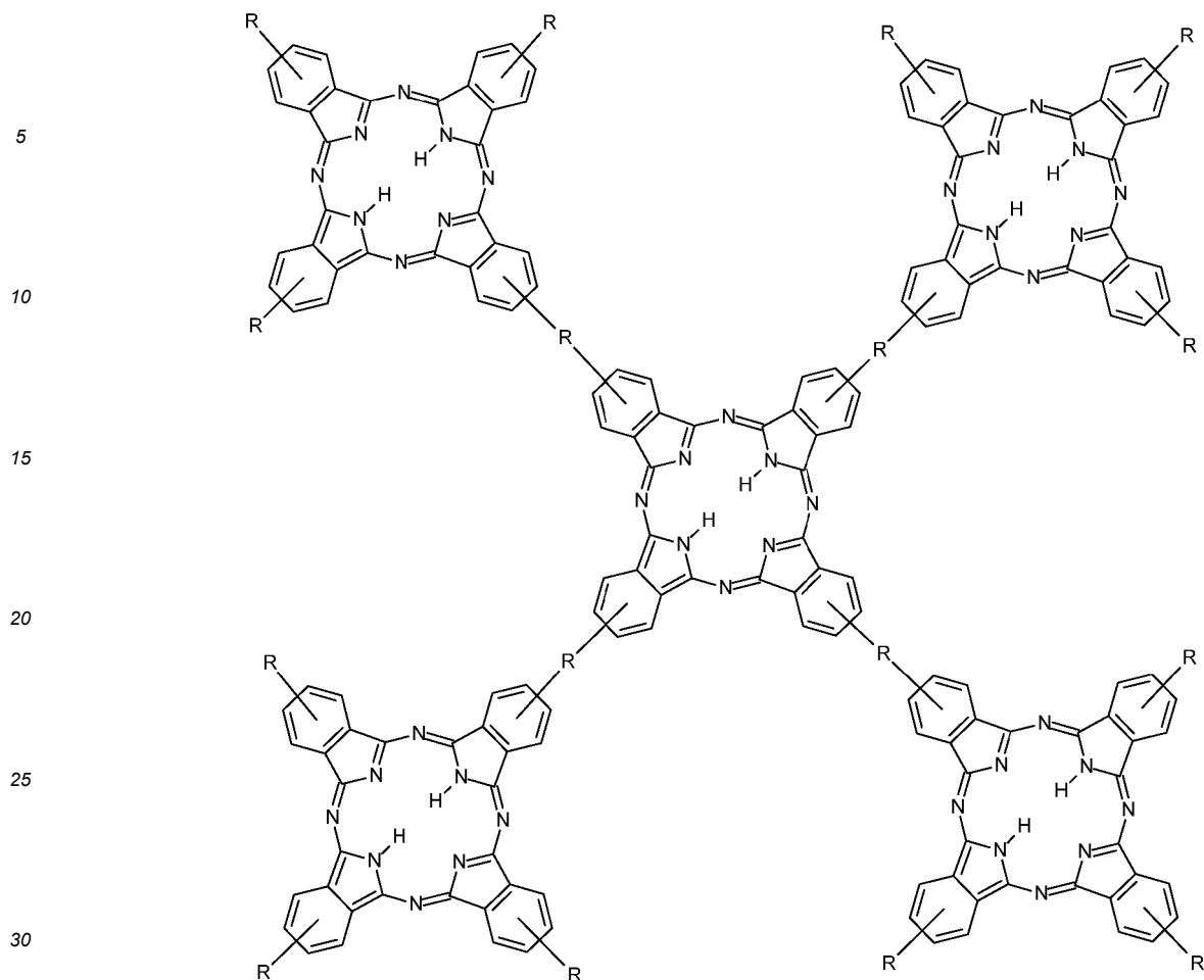
Scheme 1. Diphthalonitrile addition reaction to form a metal free phthalocyanine linked network.
