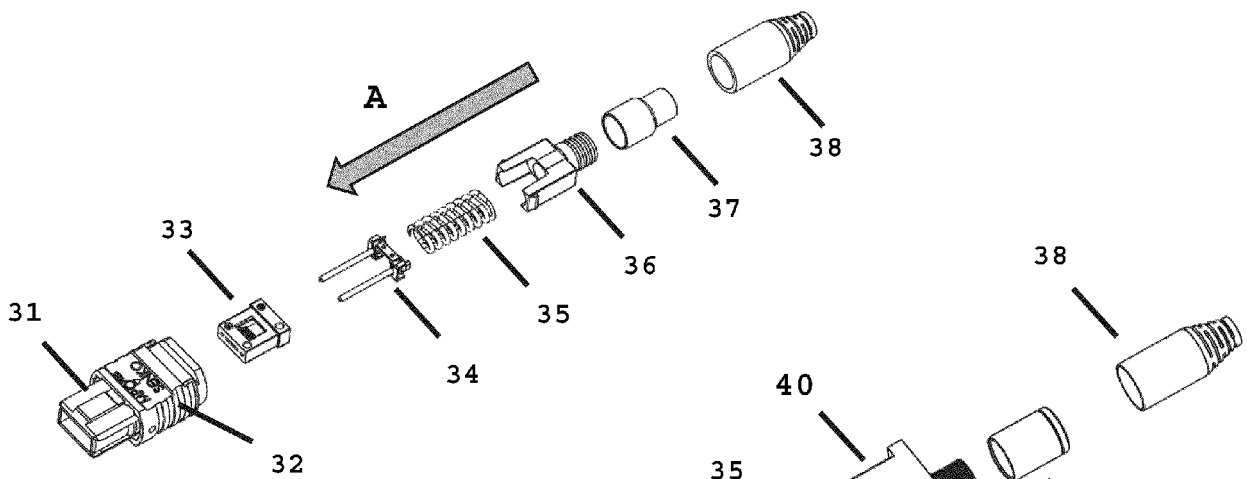
FIG. 2 (prior art)
