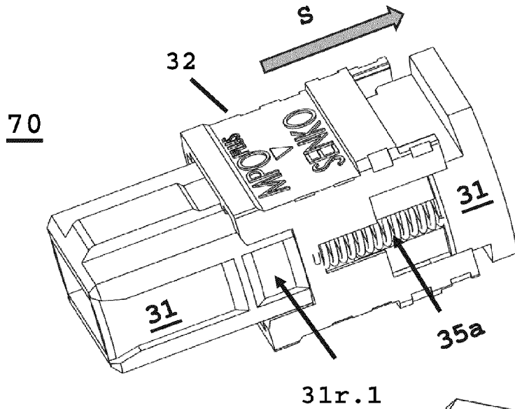
FIG. 4 (prior art)
