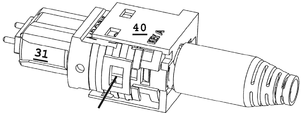
FIG. 8 40s.1
