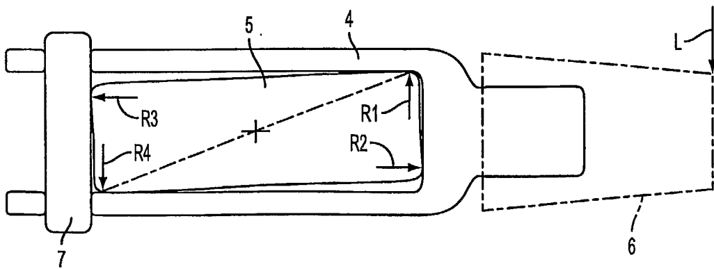
FIG. 16 (PRIOR ART)
