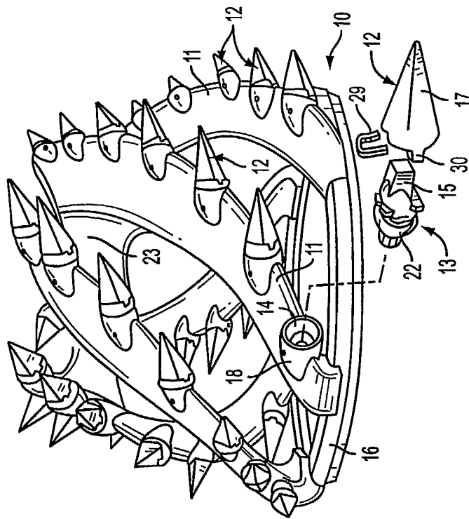
FIG. 17 (PRIOR ART)
