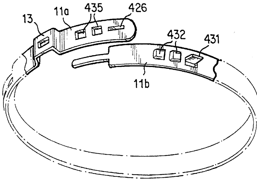
FIG. 19 PRIOR ART
