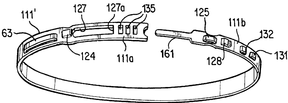
FIG. 6 PRIOR ART
