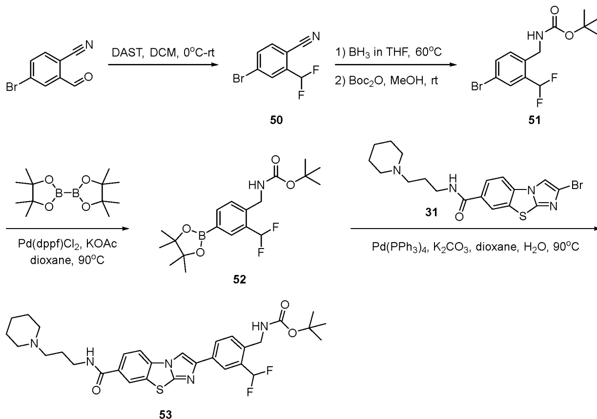
Scheme 38
