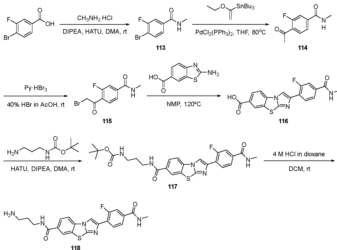
Scheme 53
