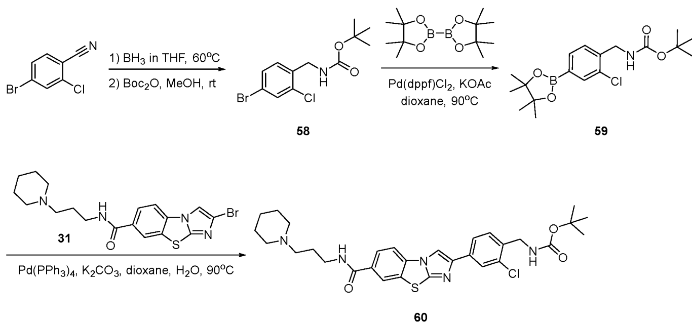
Scheme 40
