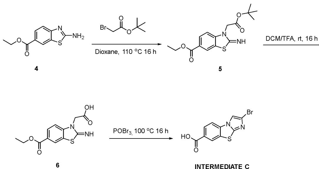
Scheme 25
