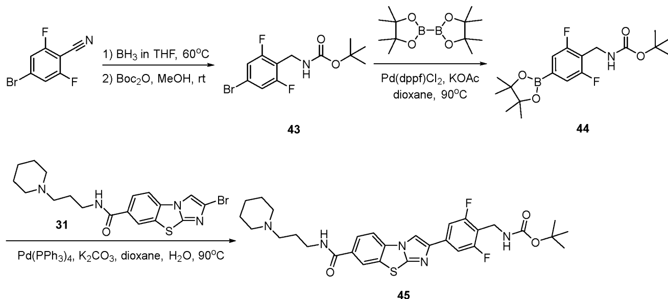
Scheme 36
