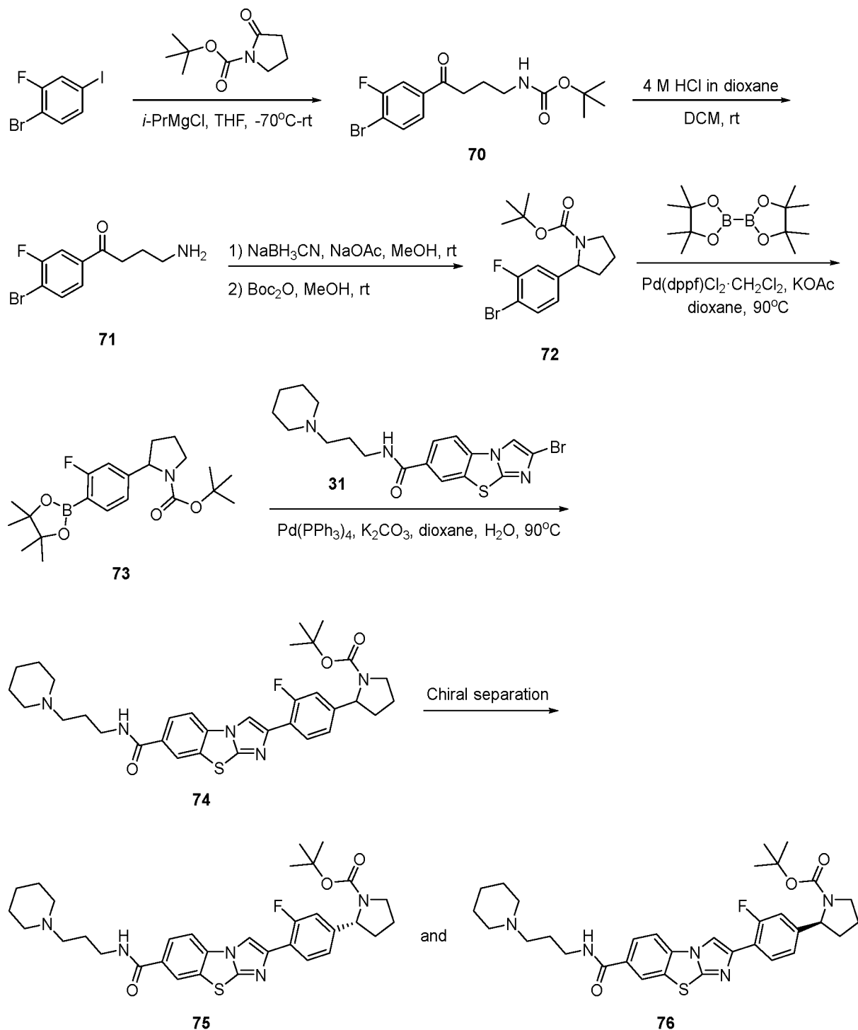
Scheme 44
