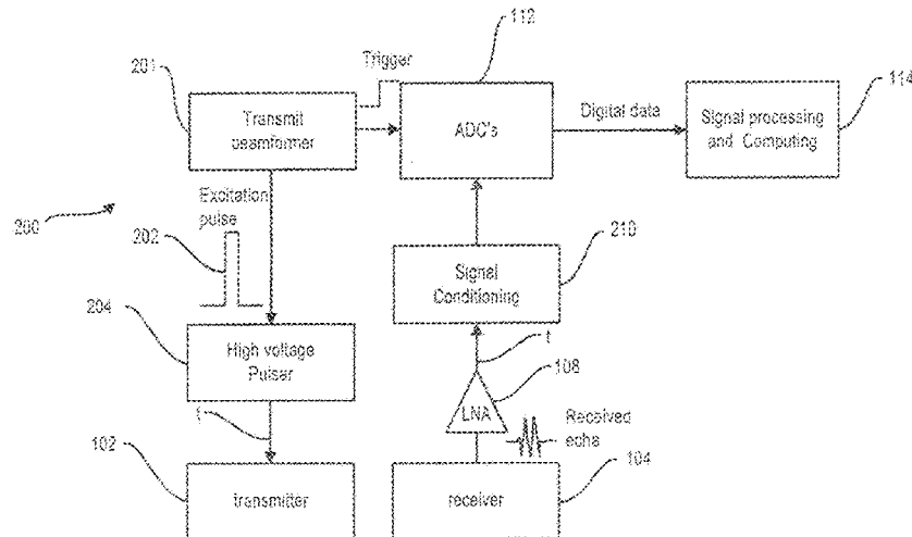
Integrated transmit and receive beamforming
