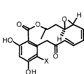
Structures of Monocillin I, Radicol and Geldanamycin
