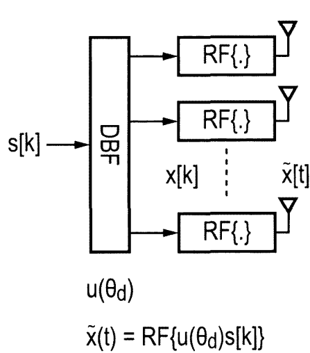
(a) Modular AAA model
