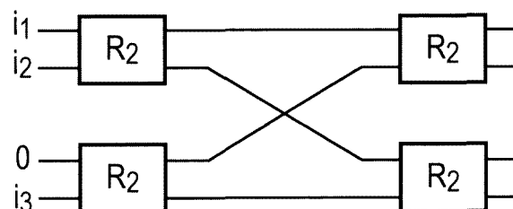
R 2 Ratrace coupler
