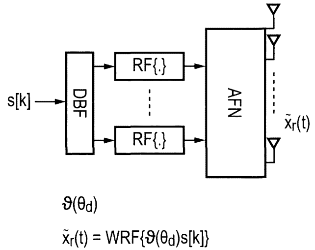
(b) Reduced dimension CFN architecture
