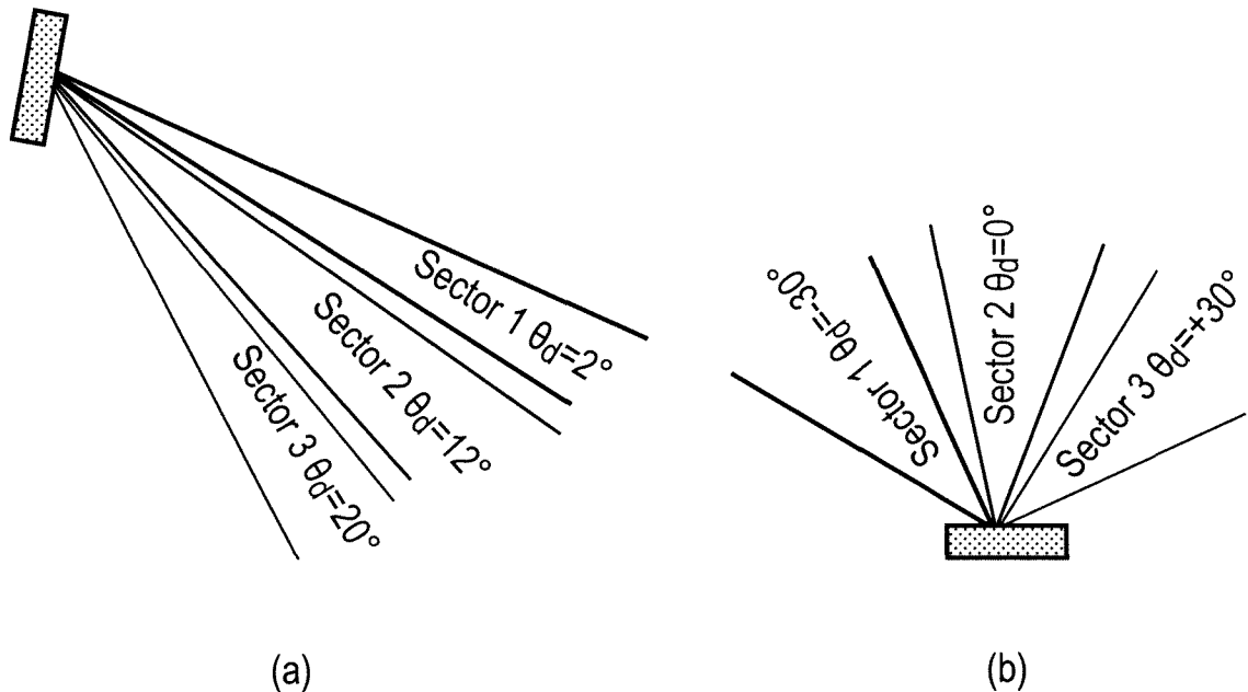
AFN cellular sectorization: (a) Macro-cell setup with narrow powerfull beams towards \theta_d (b) small cell setup with wide and orthogonal beam patterns
