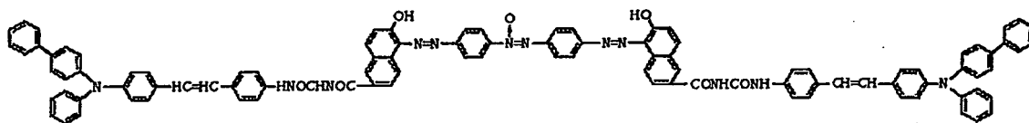
Exemplified compound (8)
