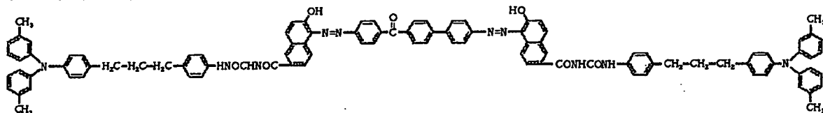
Exemplified compound (7)
