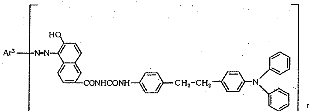
General formula (3)
