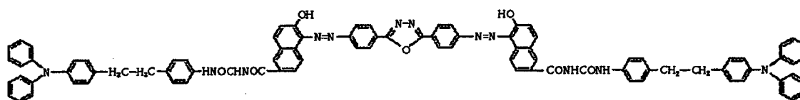
Exemplified compound (4)
