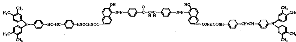
Reference compound (11)
