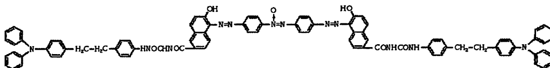
Exemplified compound (3)
