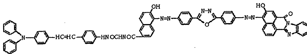
Reference compound (17)
