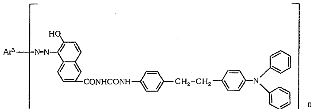
General formula (3)
