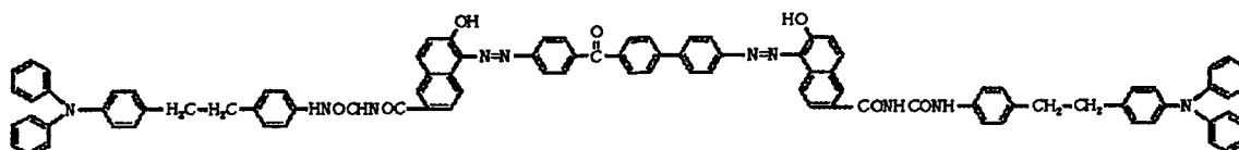
Exemplified compound (2)
