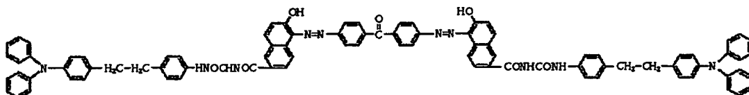
Exemplified compound (1)
