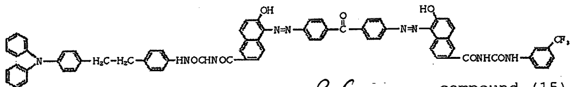
Reference compound (15)
