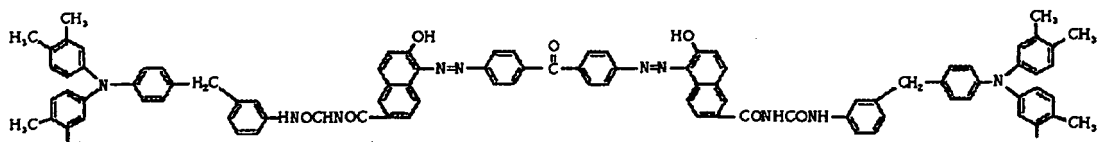
Exemplified compound (6)
