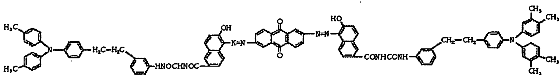
Reference compound (10)
