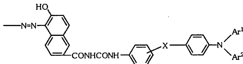
General formula (1)
