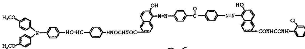
Reference compound (16)
