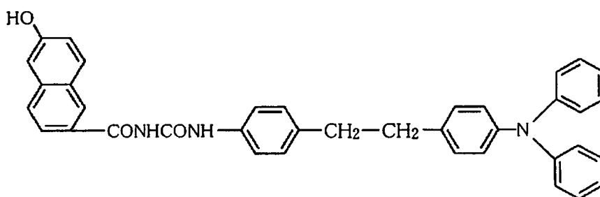
Coupler (1)
