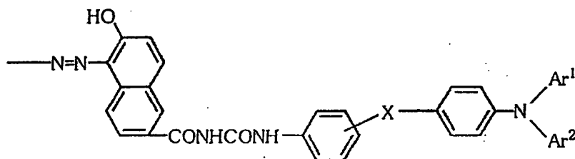
General formula (1)
