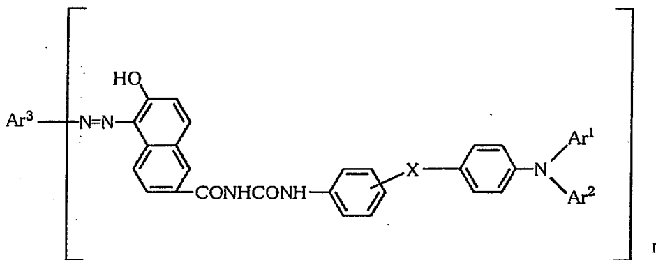
General formula (2)
