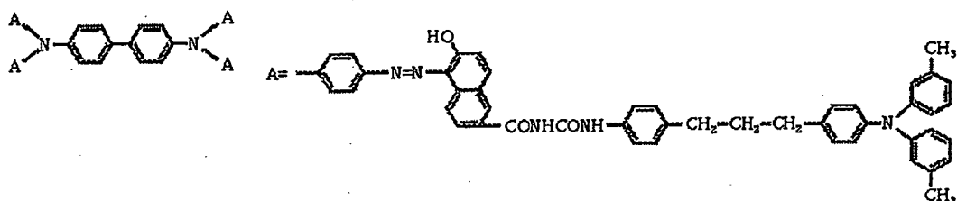
Reference compound (14)
