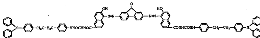
Reference compound (9)
