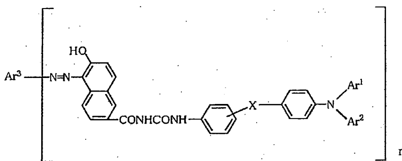
General formula (2)
