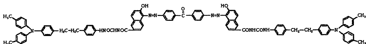
Exemplified compound (5)
