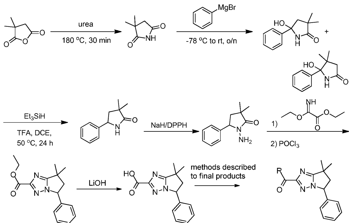
Scheme 3
