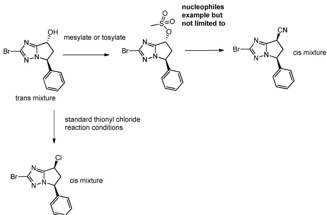
Scheme 2
