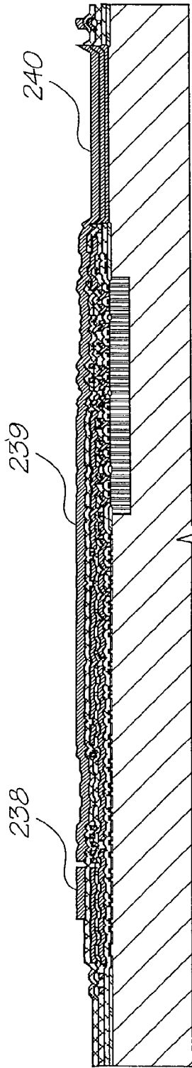
Deposit metal 3
