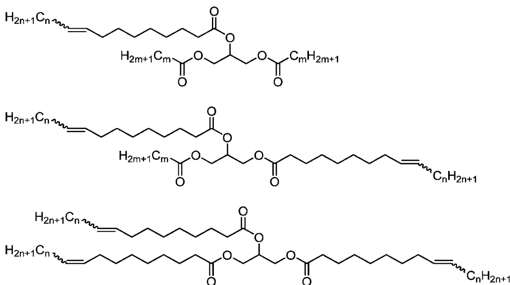
5 Scheme 4. Possible structures composing PMTAG. n=0, 2, 8 ; m=11 to 20 .
