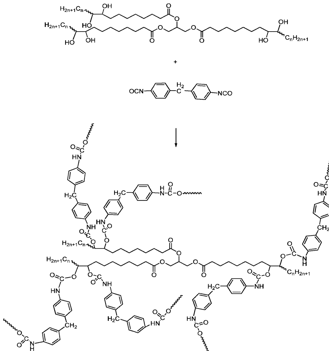
Scheme 8. Preparation of cross linked polyurethane from MDI and MTAG Polyols. Hexol structure is used as an example. n=0, 2 or 8
