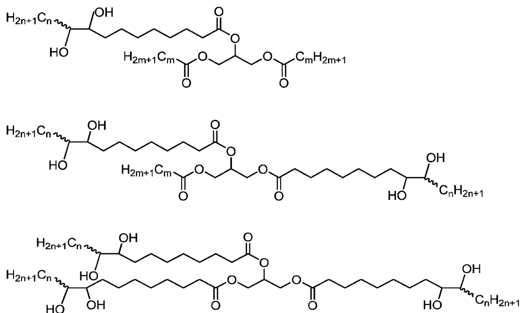
Scheme 6. Possible structures in SF- and LF-PMTAG Polyol ( n=0, 2, 8 ; m=11 to 20 )
