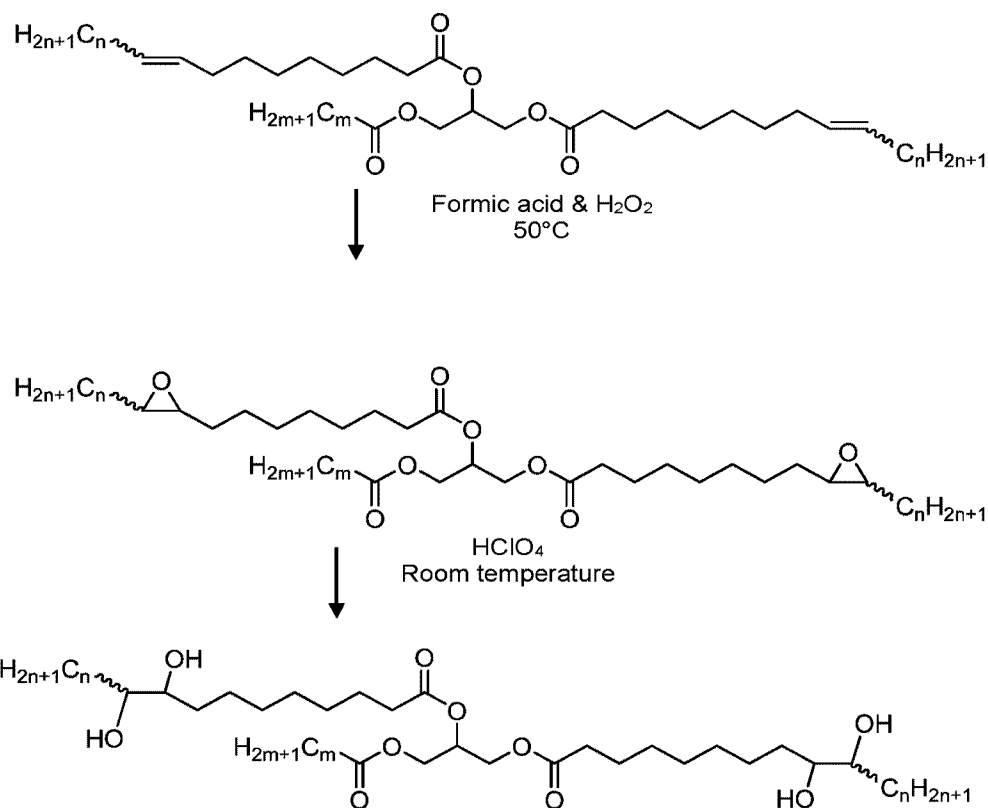
Scheme 5. Synthesis of PMTAG Polyol ( n=0, 2, 8 ; m=11 to 20 )
