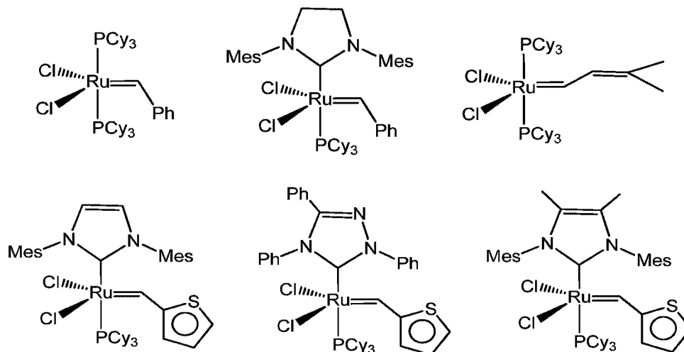
Scheme 2. Structures of few metathesis catalysts.
