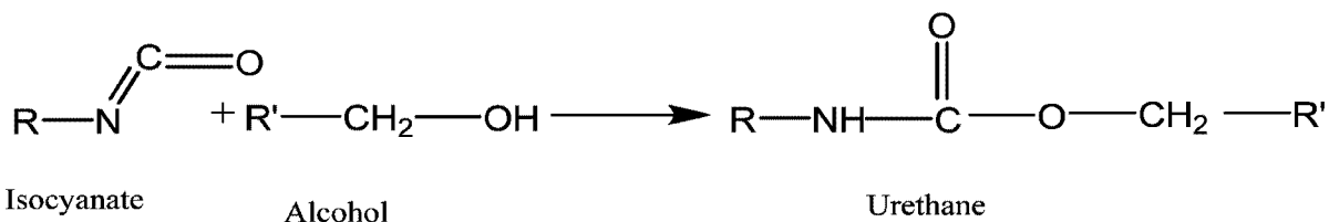
Scheme 7. General formation of urethane linkage between isocyanate group and OH group
