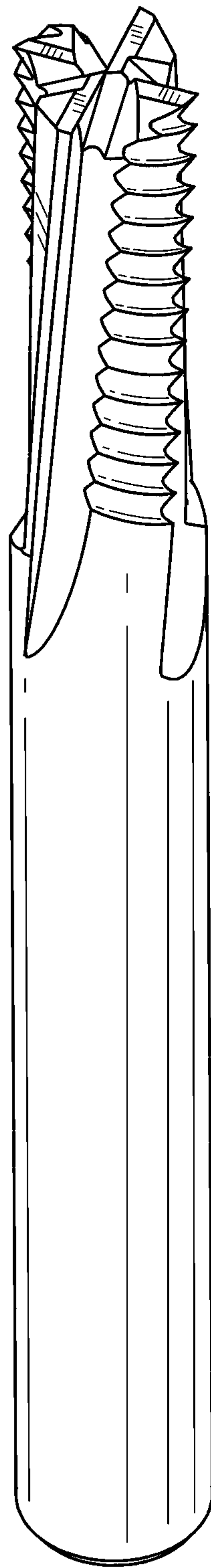
立體圖2
