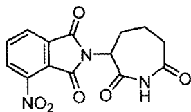
Compound 2
