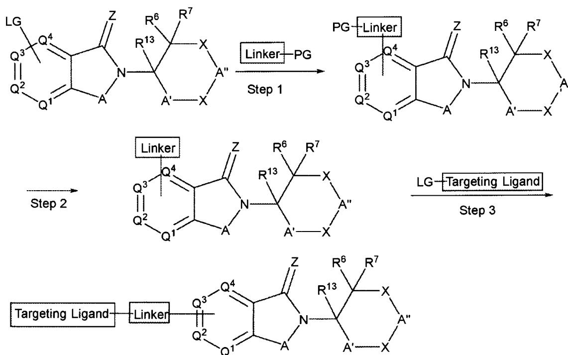
Scheme 6
