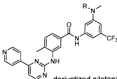
derivatized nilotinib
