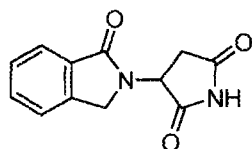
Compound 1
