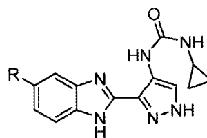
derivatized AT-9283
