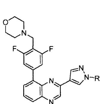
derivatized NVP-BSK805
