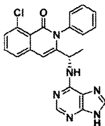
Compound 292
