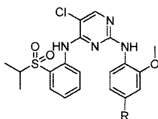
derivatized TAE684
