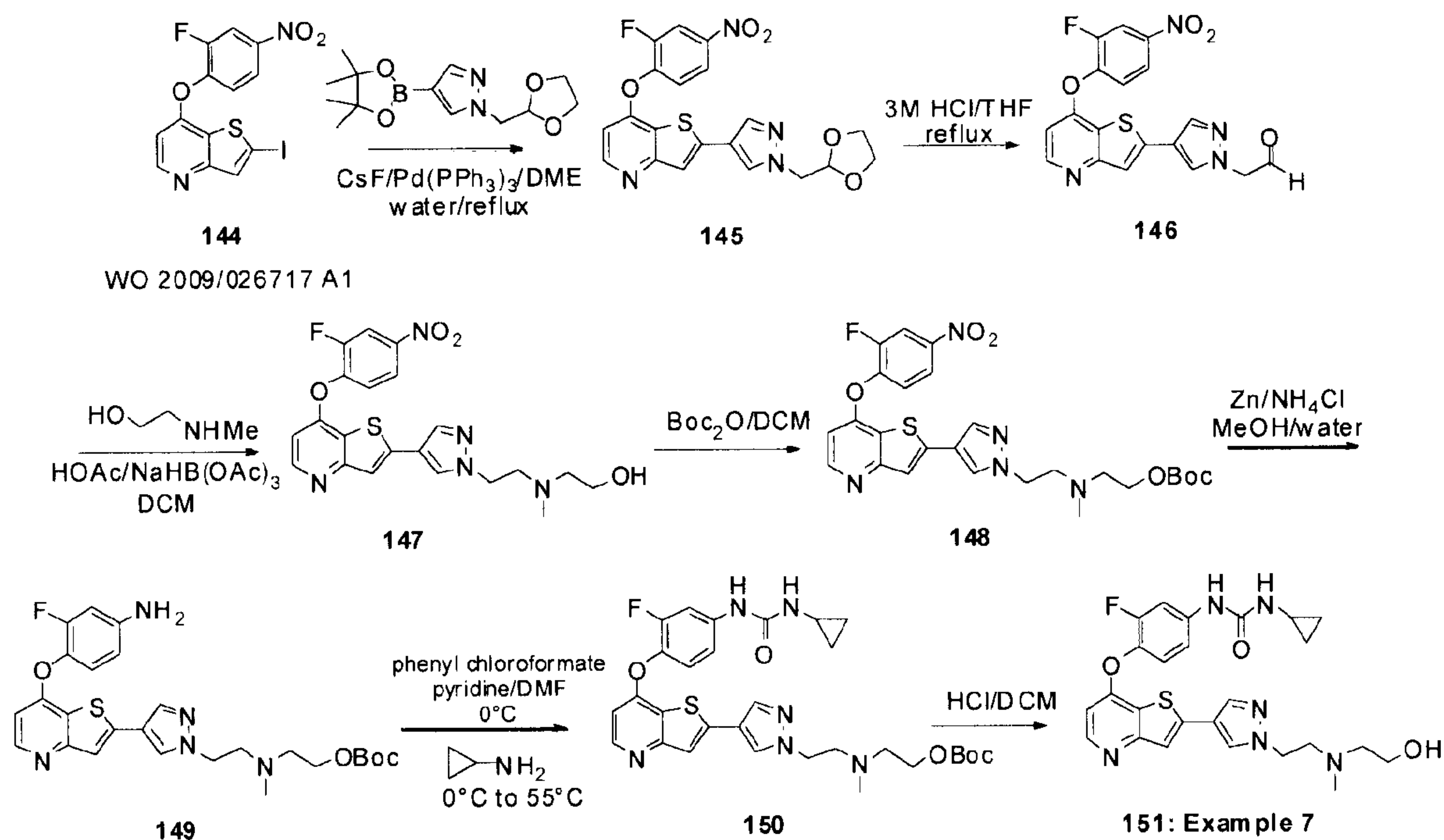
Scheme 6
