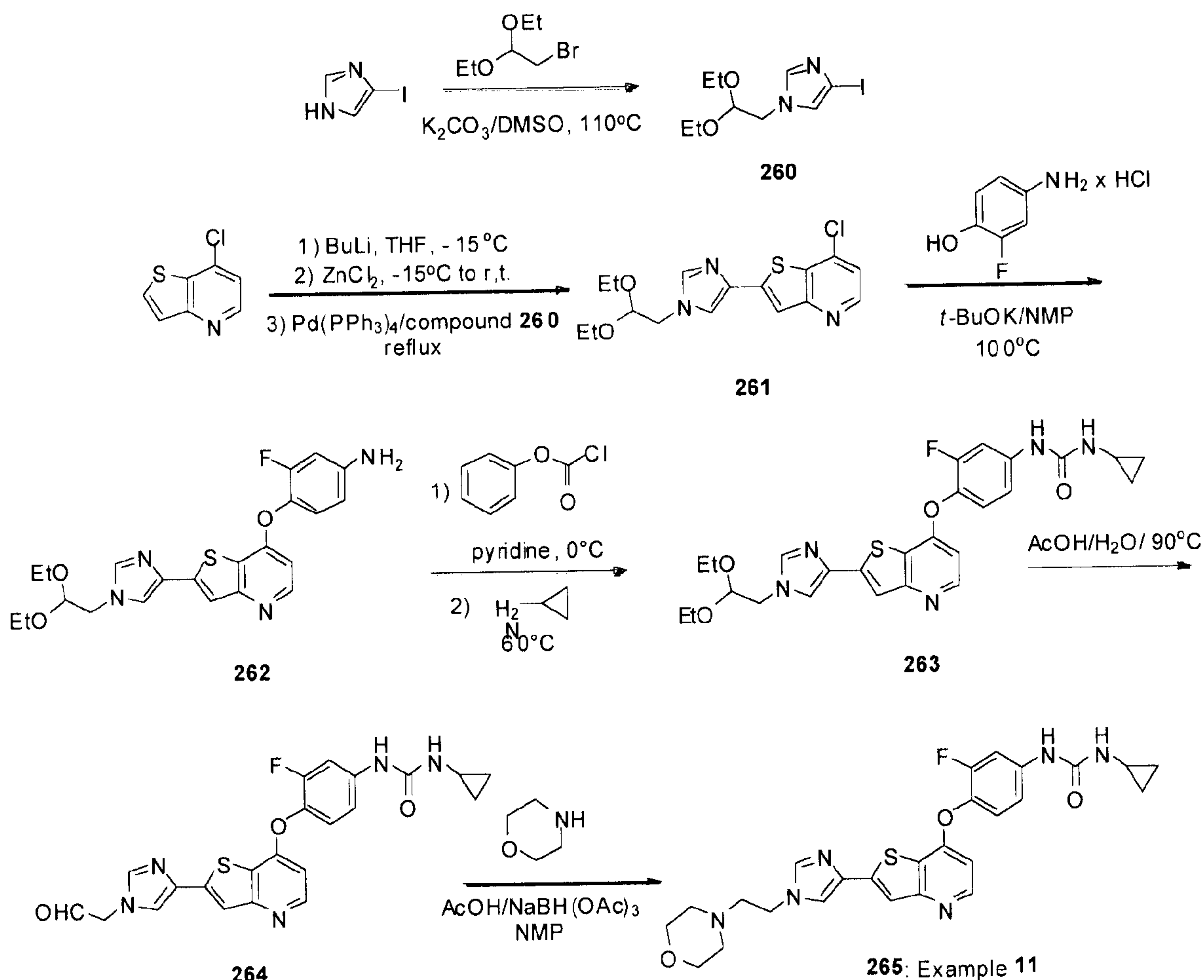
Scheme 9
