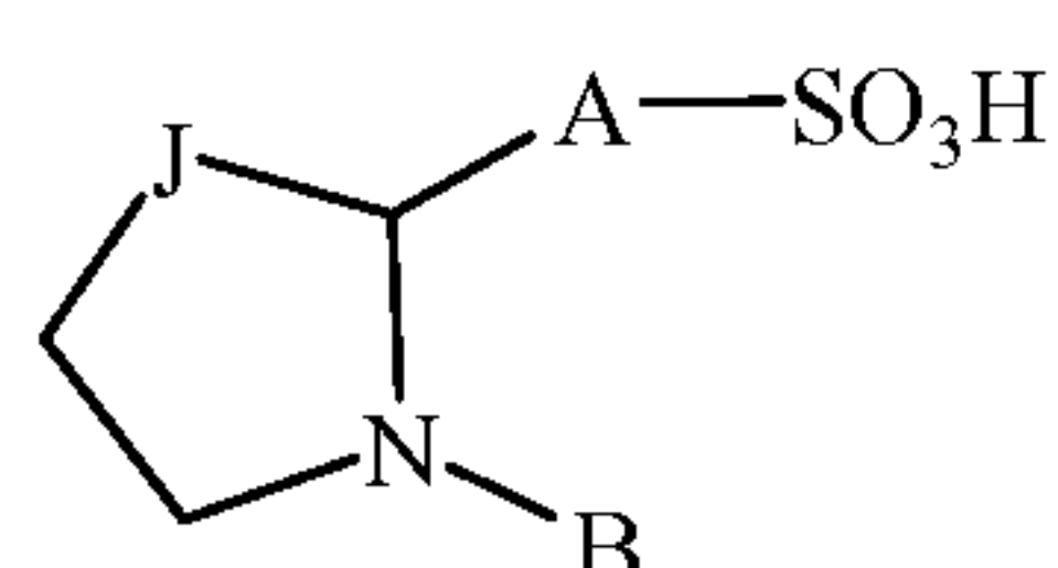
Sulfonic Acid
