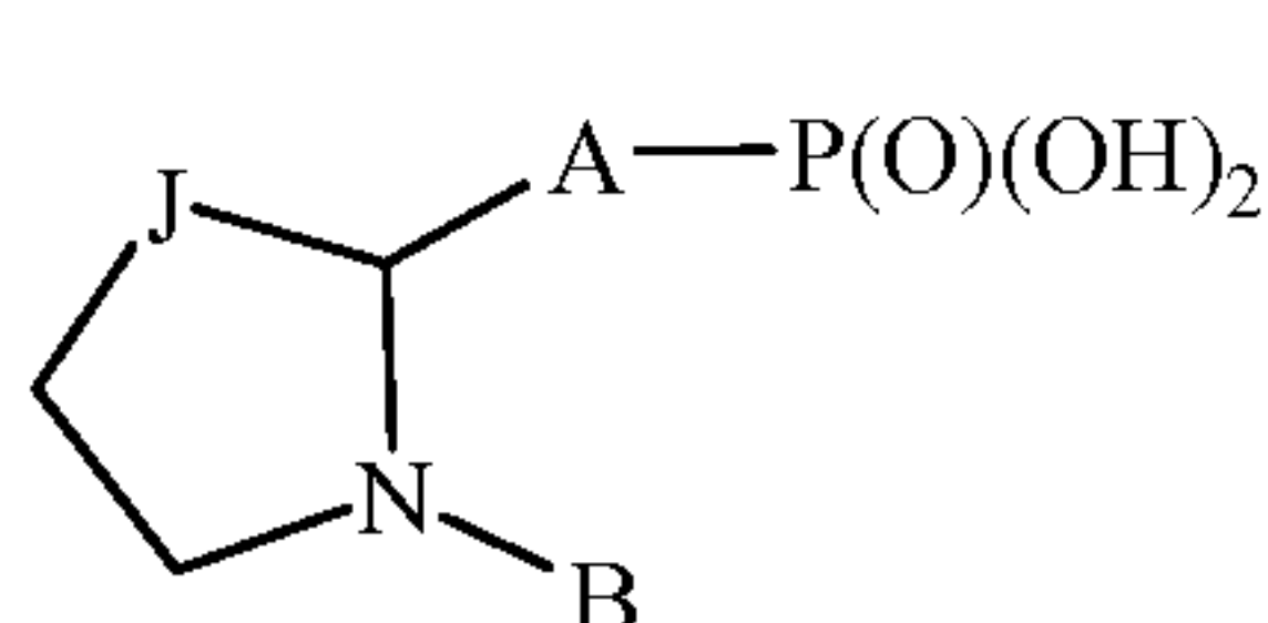
Phosponic Acid
