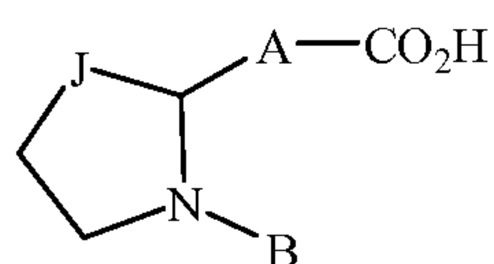
Carboxylic Acid
