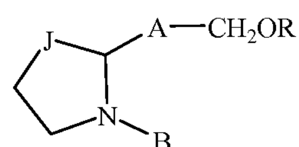
Ether
