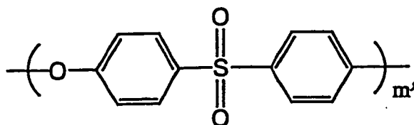
Chemical Formula (14)
