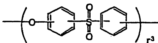
Chemical formula (10)
