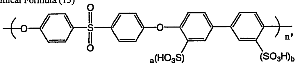
Chemical Formula (15)
