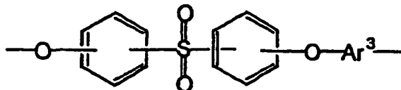
Chemical Formula (4)
