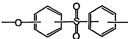
Chemical Formula (3)
