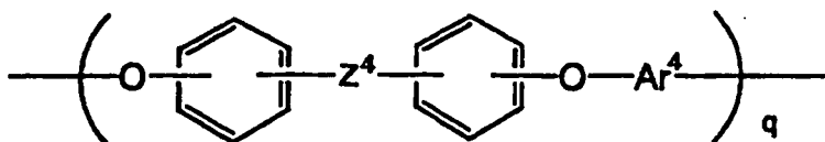
Chemical Formula (7)
