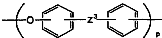
Chemical Formula (6)
