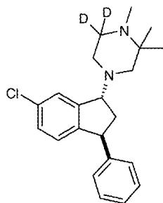
Compound (III)
