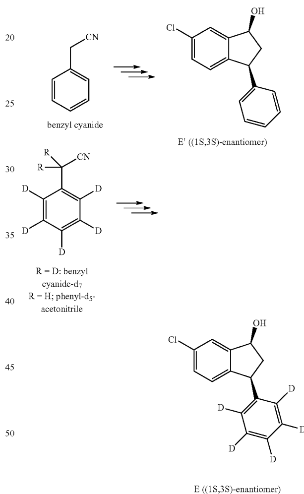
Scheme 4. Exemplary synthesis of intermediates E and E'.
