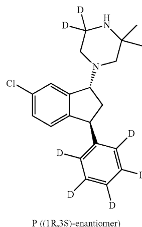
P ((1R,3S)-enantiomer)
