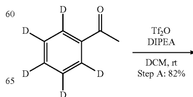
Scheme 14. Synthesis of Compound (XV)
