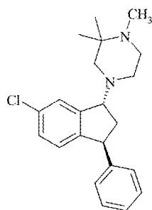
Compound (VI)
