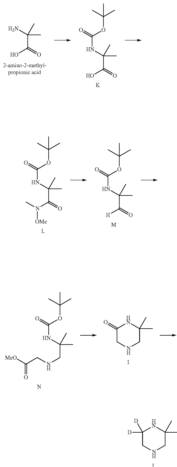
Scheme 7. Alternative exemplary synthesis of intermediate J.
