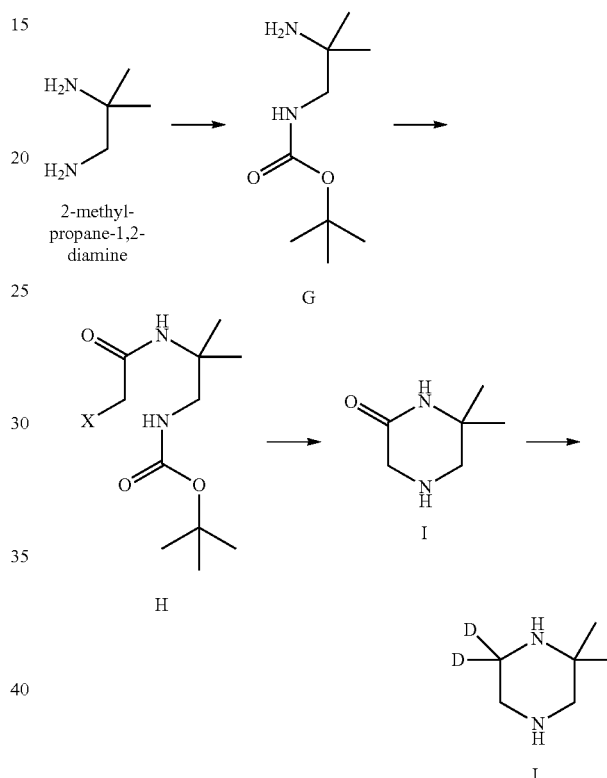
Scheme 6. Exemplary synthesis of intermediate J.
