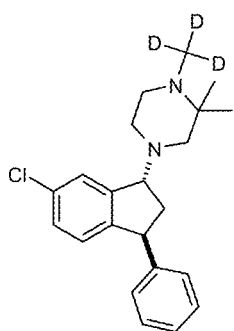
Compound (I)
