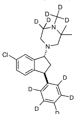
Compound (VI)
