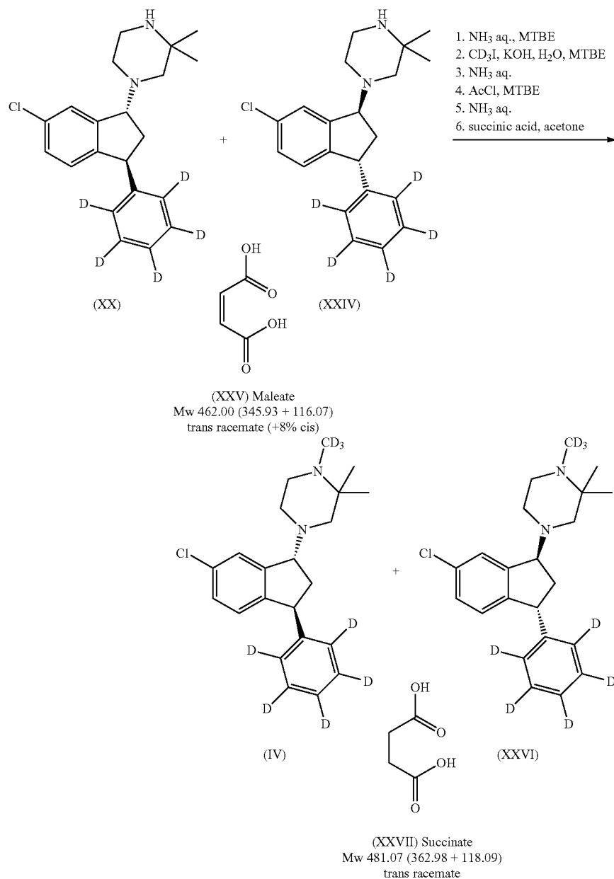
Scheme 17: Synthesis of rac-trans-1-(6-chloro-3-phenyl( d_5 )-indan-1-yl)-1( d_3 ), 2,2-trimethyl-piperazine succinate.
