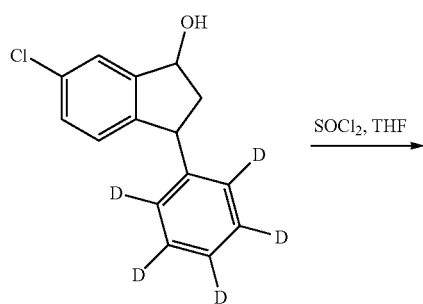
(XXII) cis racemate Mw 249.75 C_{15}H_8ClOD_5
