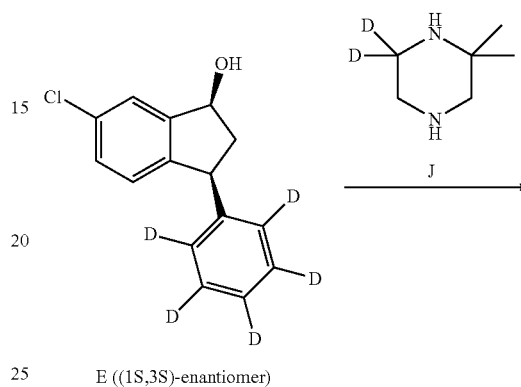
E ((1S,3S)-enantiomer)
