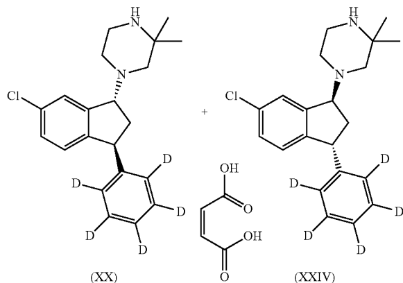
(XXV) maleate Mw 462.00 (345.93 + 116.07) trans racemate (+8% cis)
