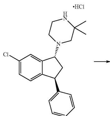
1-((1 R ,3 S )-6-Chloro-3-phenyl-indan-1-yl)-3,3-dimethyl-piperazine hydrochloride (Compound XI) hydrochloride
