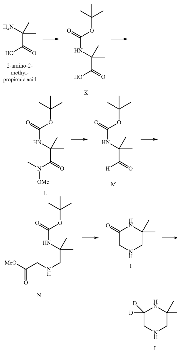
Scheme 11. Synthesis of intermediate J.
