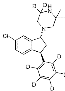
(XXI)
