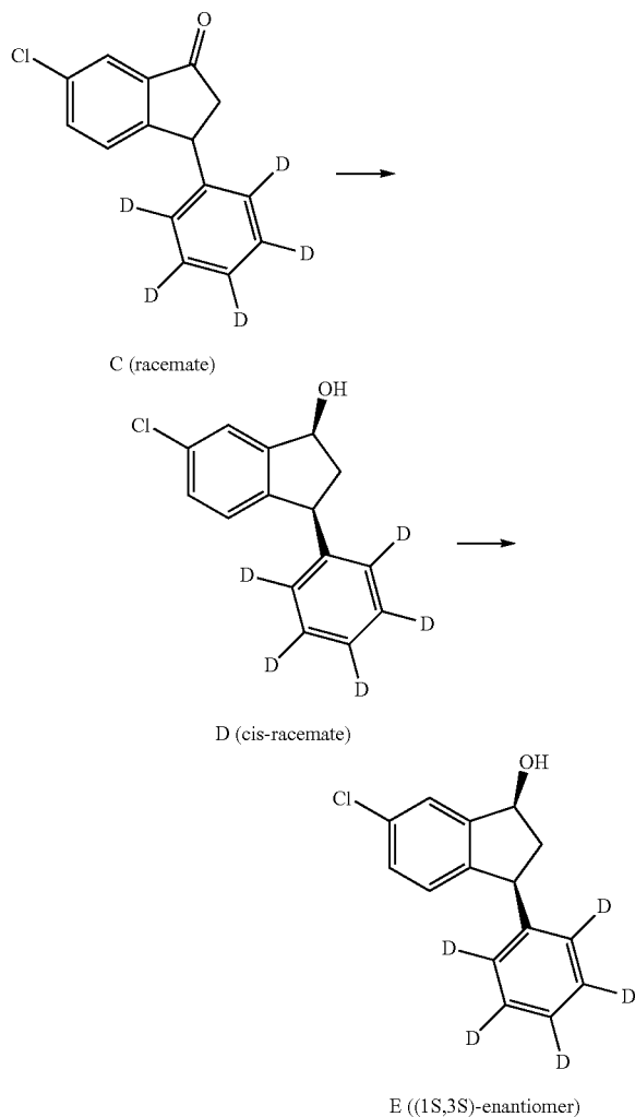
Scheme 2. Exemplary synthesis of intermediate E.
