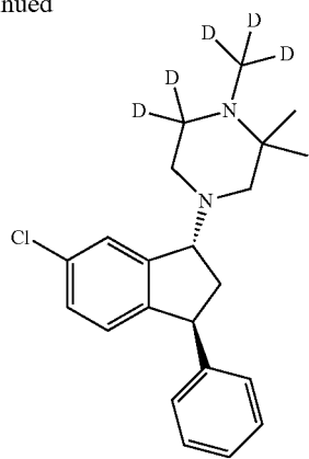
Compound (V)
