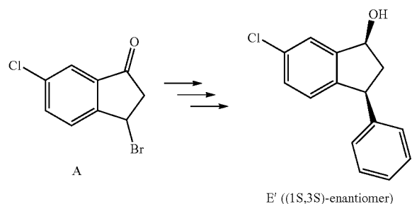
Scheme 3. Exemplary synthesis of intermediate E'.
