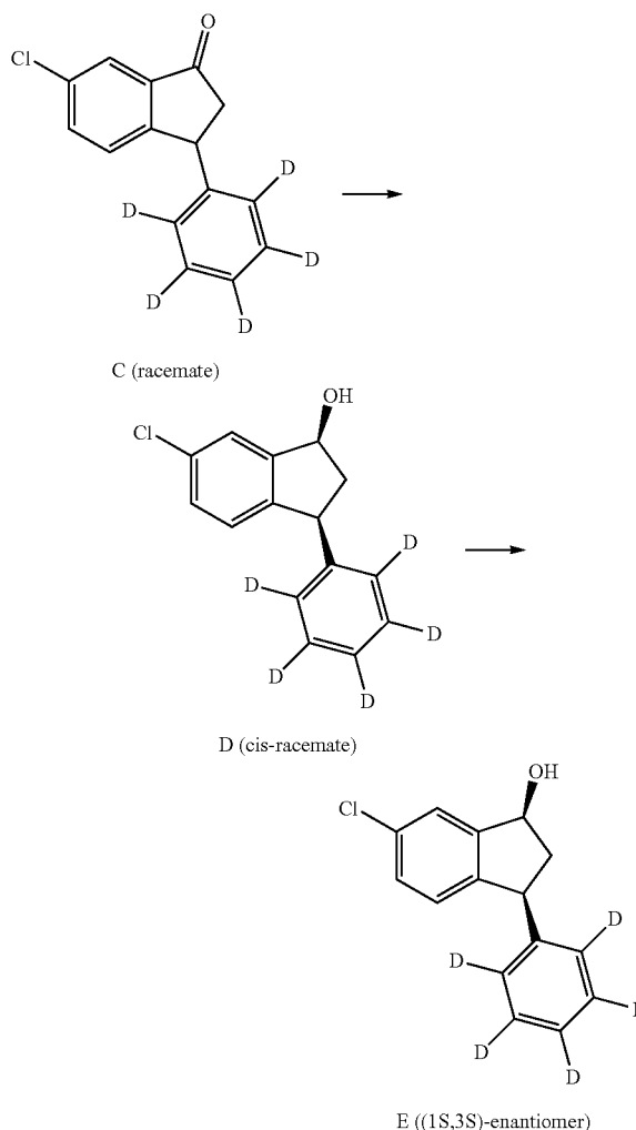
Scheme 10. Synthesis and resolution of Compound E.
