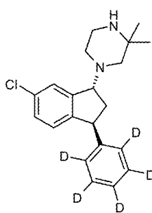
(XX)
