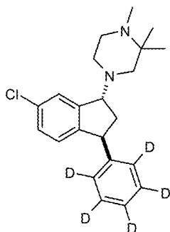
Compound (II)
