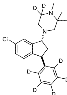
Compound (VII)
