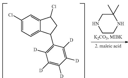
(XXIII) cis racemate (+15% trans) Mw 268.20 C_{15}H_7Cl_2D_5
