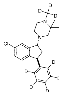
Compound (IV)
