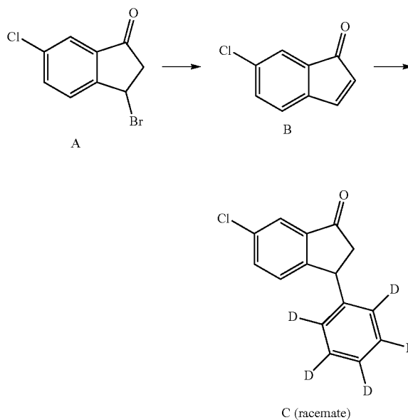
Scheme 1. Exemplary synthesis of intermediate C.
