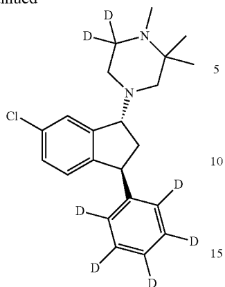
Compound (VII)
