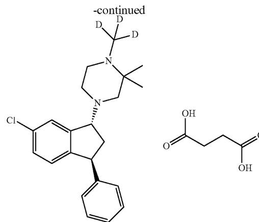
Compound (I) butanedioic acid salt
