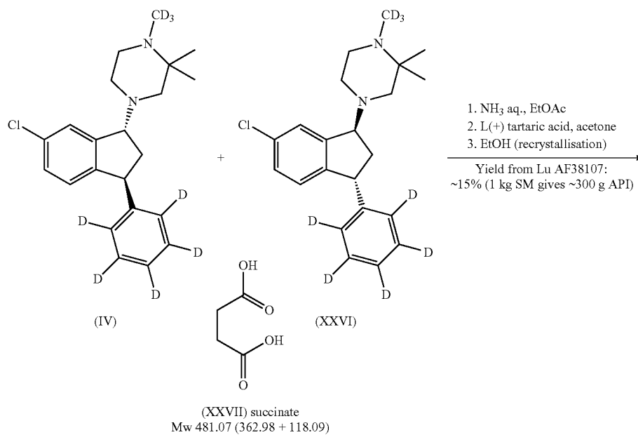
Scheme 18: Synthesis of 4-((1R,3S)-6-chloro-3-phenyl(d 5 )-indan-1-yl)-1-(d 3 ),2,2-trimethylpiperazine L(+)-hydrogen tartrate.
