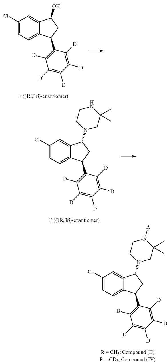
Scheme 5.
