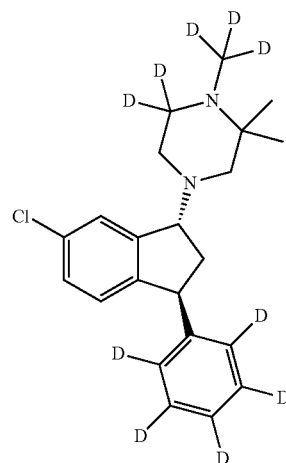
Compound (VI)
