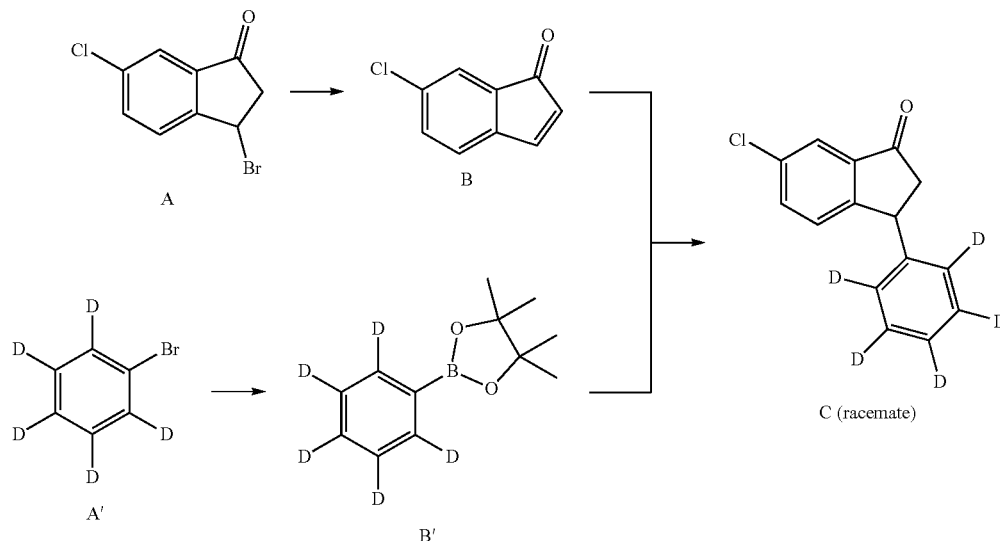
Scheme 9. Synthesis of Compound C.
