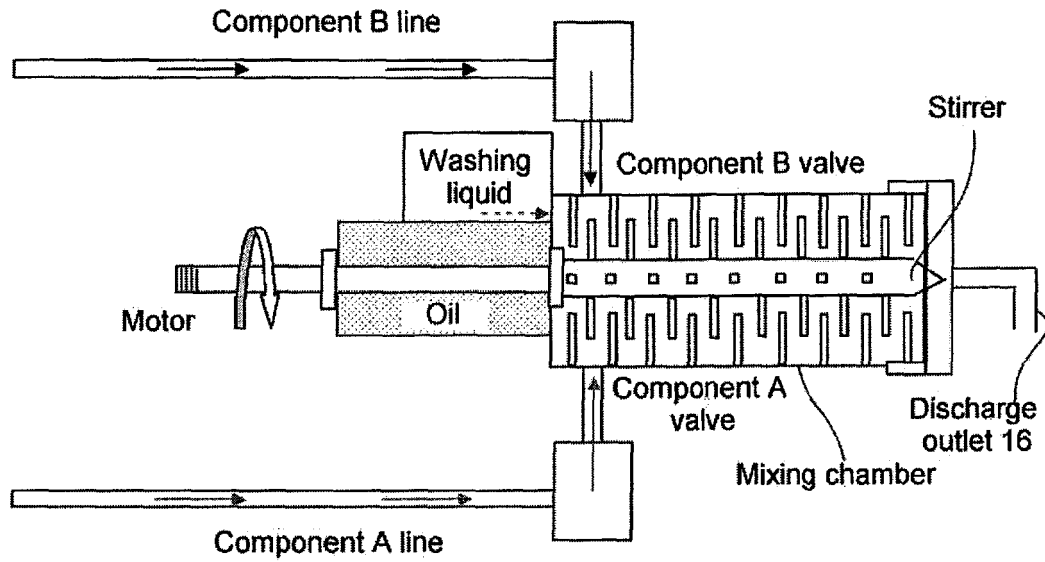
Mixing and discharging part 15
