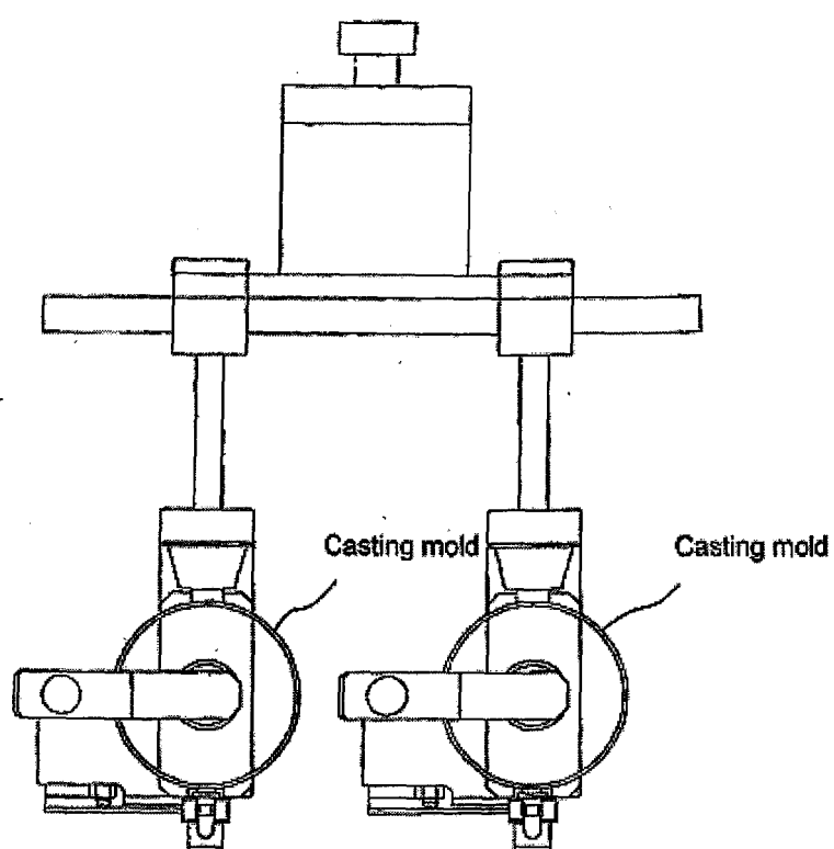
Conveying pallet 70
