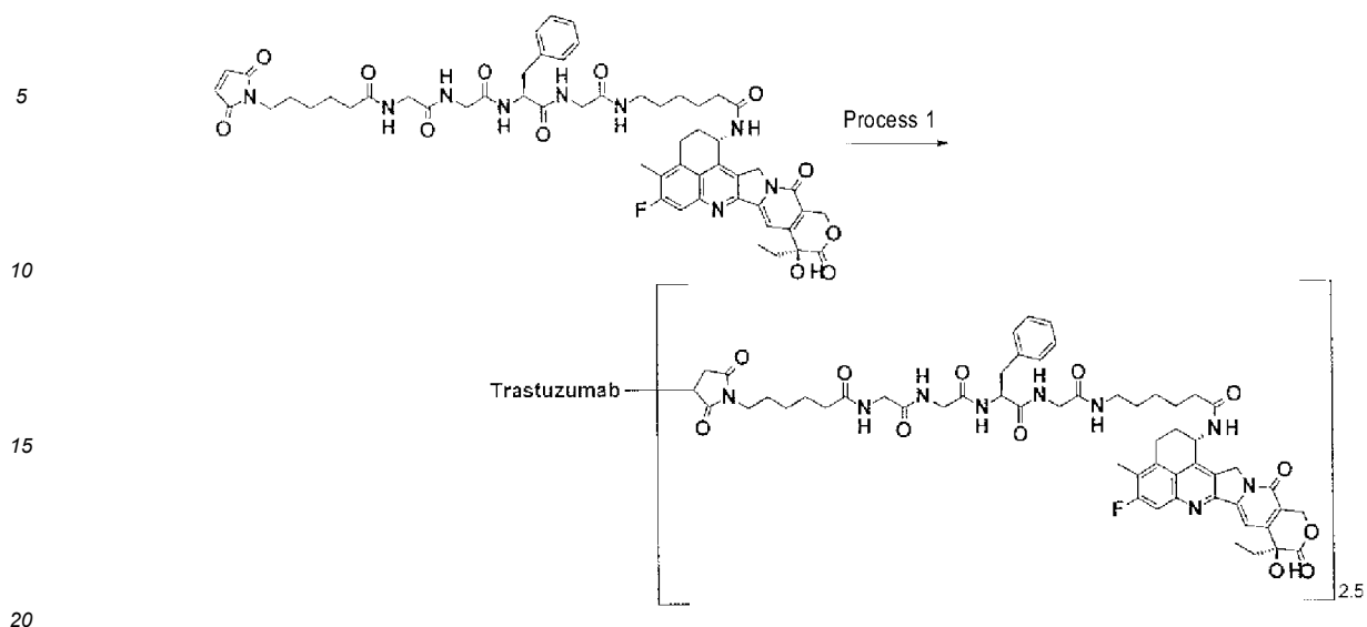
Process 1: Antibody-drug conjugate (25)
