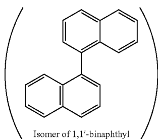
Isomer of 1,1'-binaphthyl
