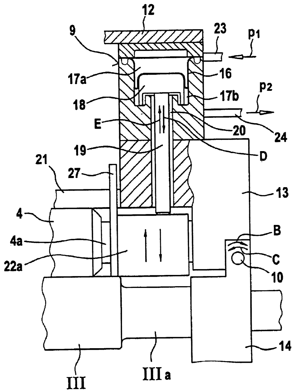
Fig. 2 Section K-K
