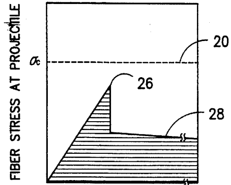
DEFLECTION (HEIGHT OF PYRAMID)
