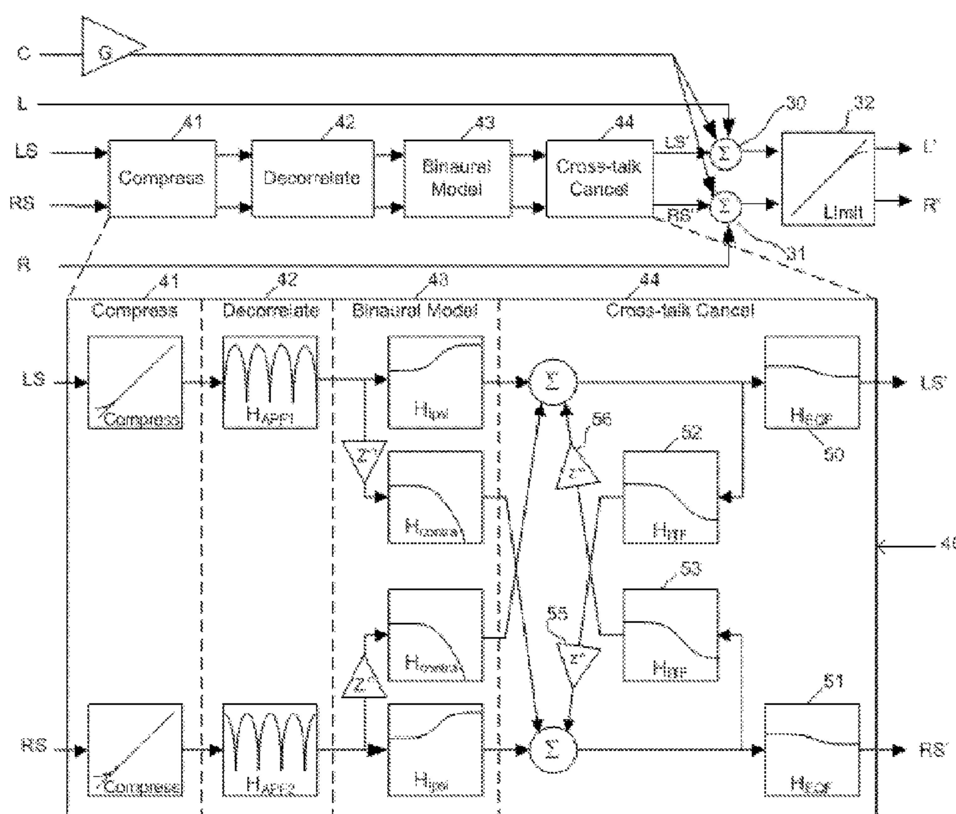
Figure 3 - Virtualizer Block Diagram
