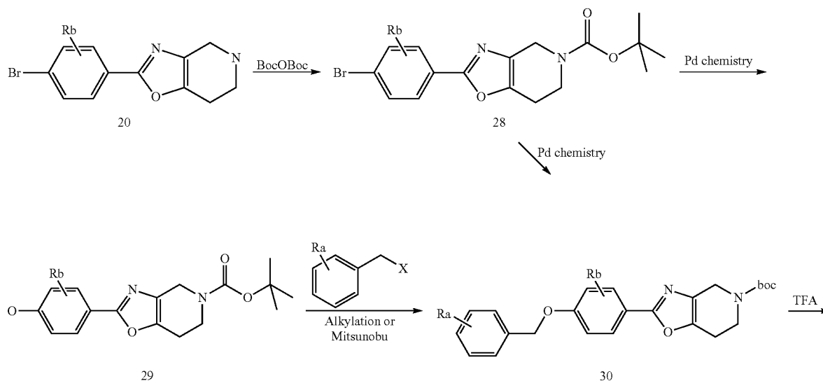
Scheme 7. Route E for the synthesis of compounds 2
