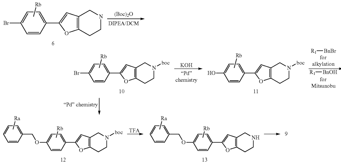
Scheme 3. Route B to compounds 1
