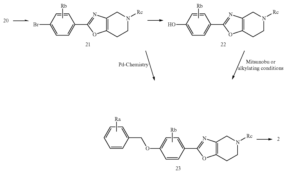
Scheme 5. Route C to compounds 2.
