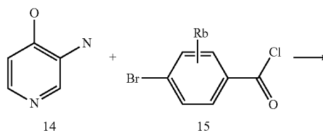
Scheme 4. Synthesis of compounds 20.
