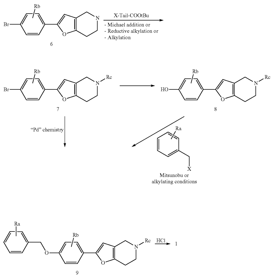
Scheme 2. Route A to compounds 1
