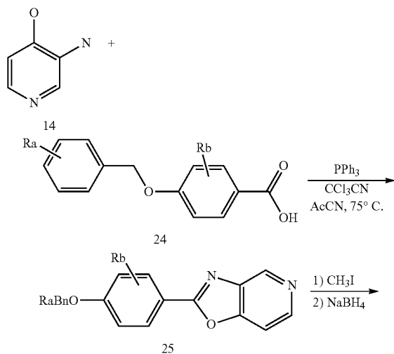
Scheme 6. Route D to compounds 2.
