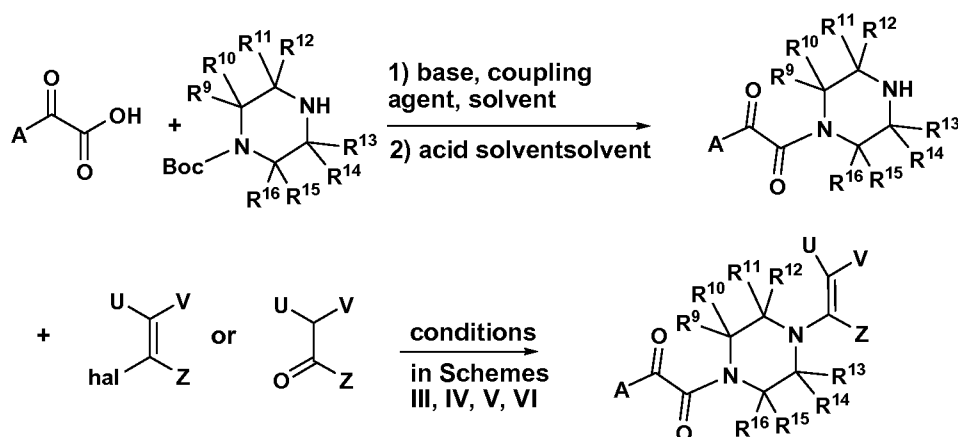
Scheme IX
