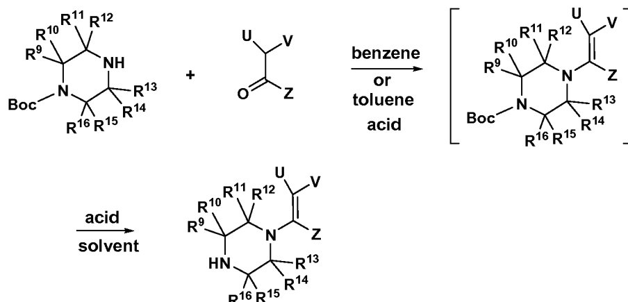
Scheme V
