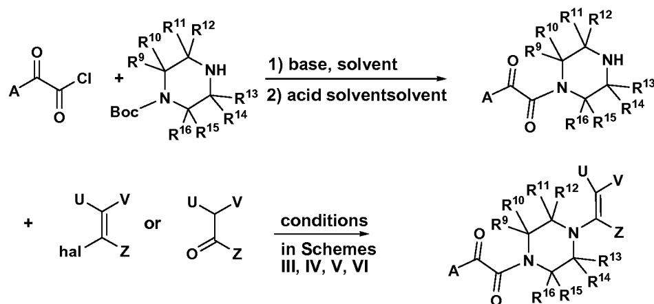
Scheme VII
