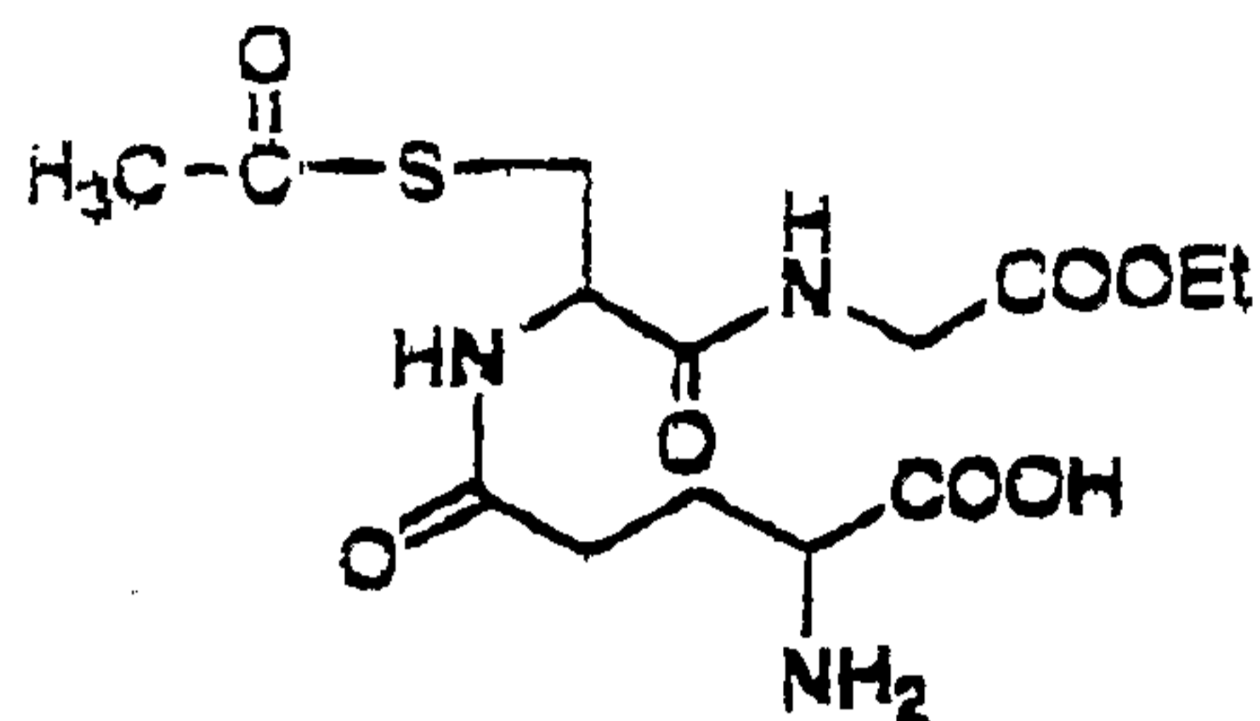
S-Acetylglutathione ethyl ester (S-Ac-GSH-OEt)
