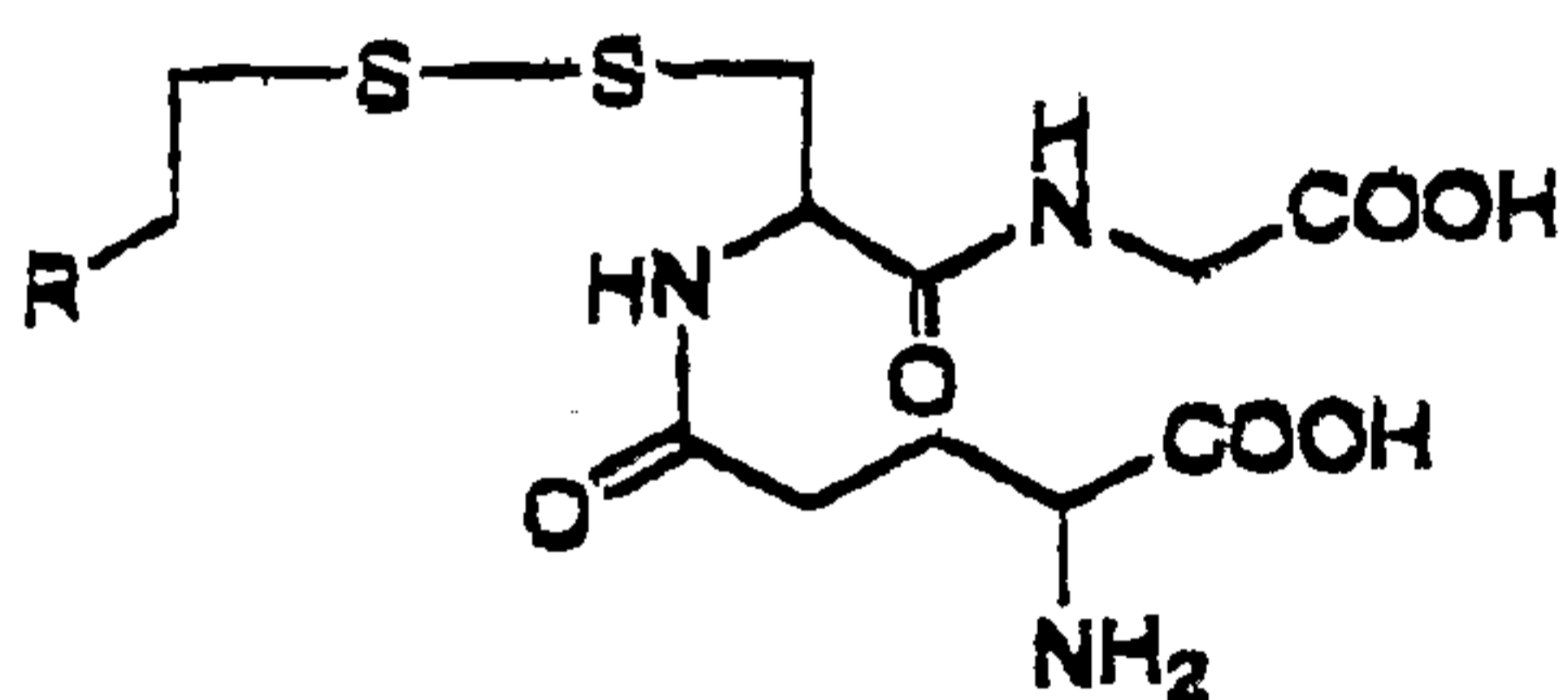
GSSMA (R = NH 2 )
