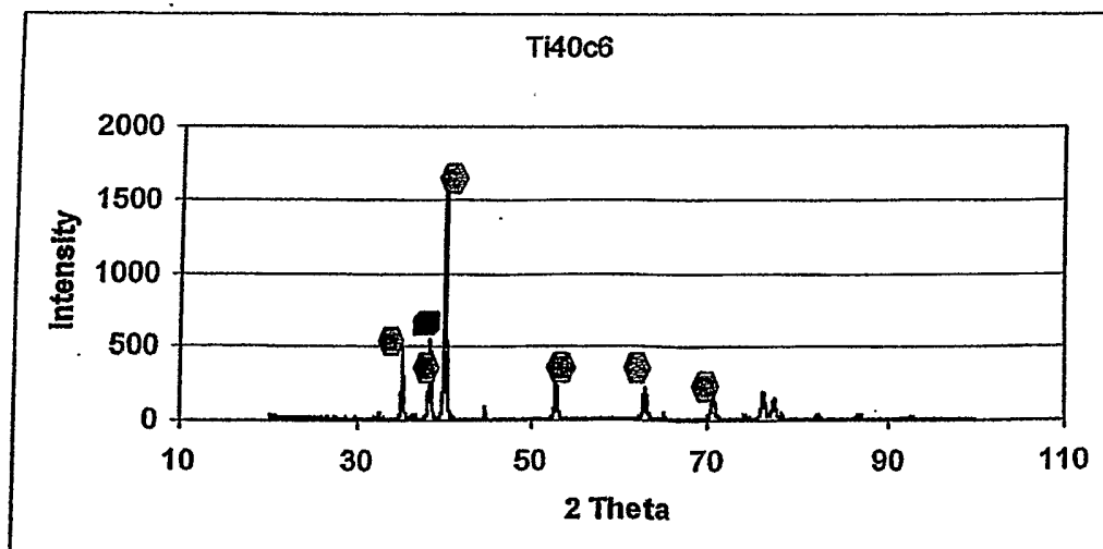
XRD spectrum of the mechanically alloyed powder of composition 6
