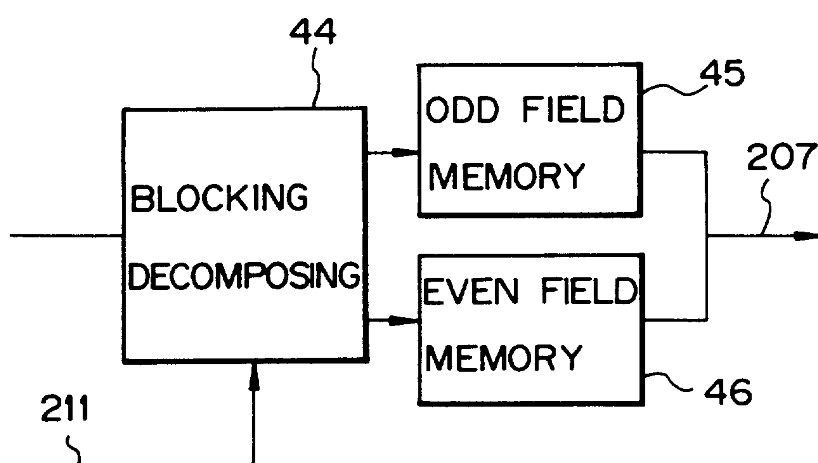
BLOCKING DECOMPOSING SECTION
