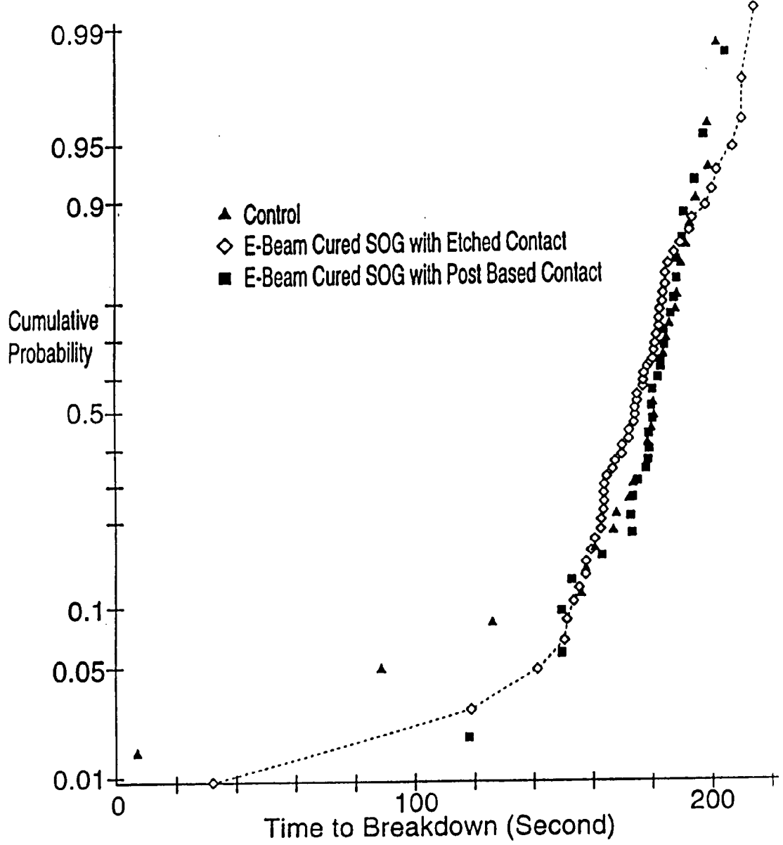
FIG. 12 QBD of Gate Oxide with TEOS Dielectric and E-Beam Cured SOG
