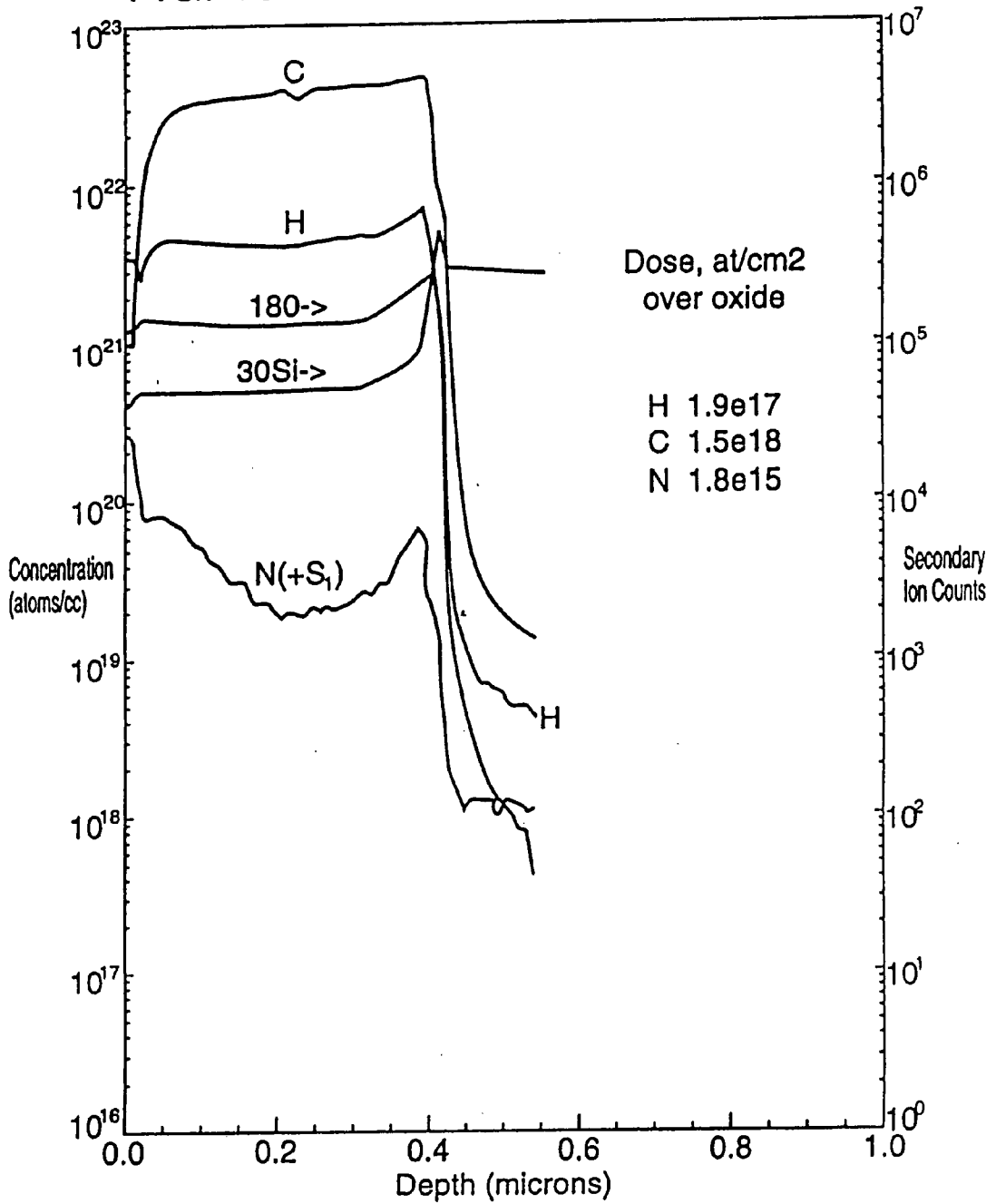
FIG. 13 SIMS Profile Analysis
