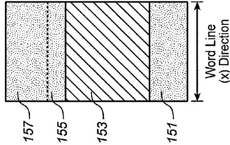
FIG. 6C (Section C-C)
