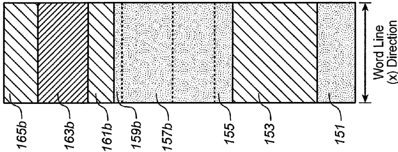
FIG. 6B (Section B-B)
