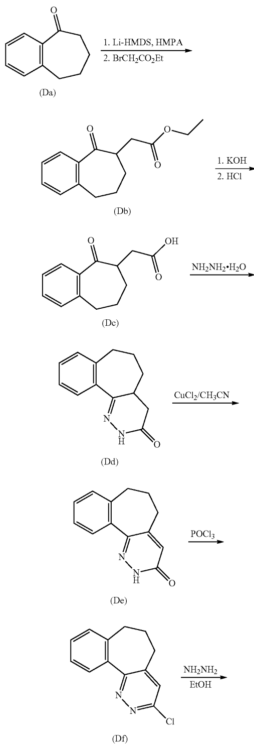
REACTION SCHEME 3
