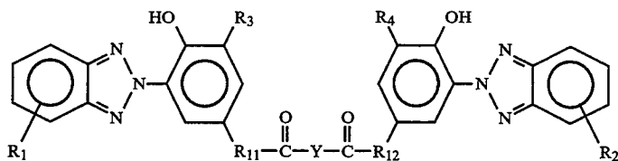
Compound 1-c
