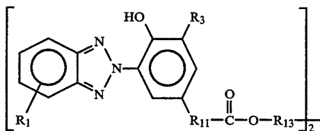
Compound 2
