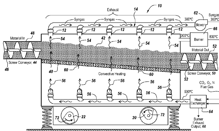
Fig. 3 (Prior Art)
