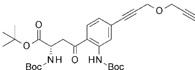
[Compound 31]
