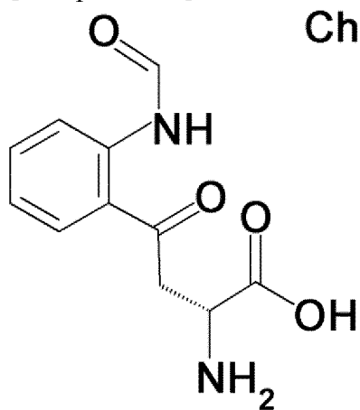
[Compound 22]
