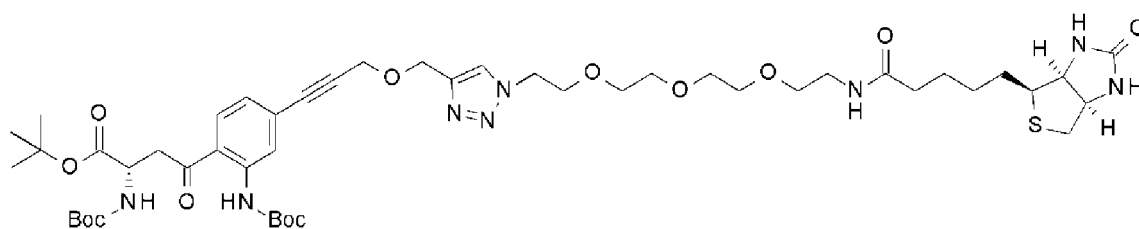
[Compound 32]
