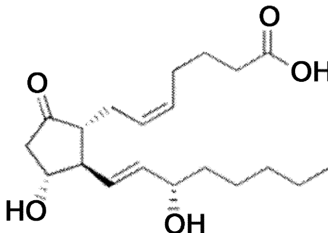
[Compound 5]
