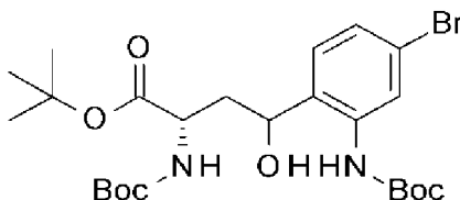
[Compound 28]
