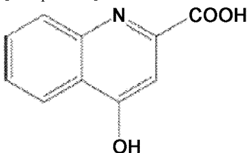
[Compound 4]
