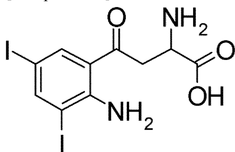
[Compound 23]
