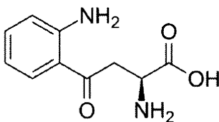
[Compound 1]
