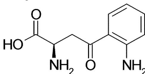
D-Kynurenine
