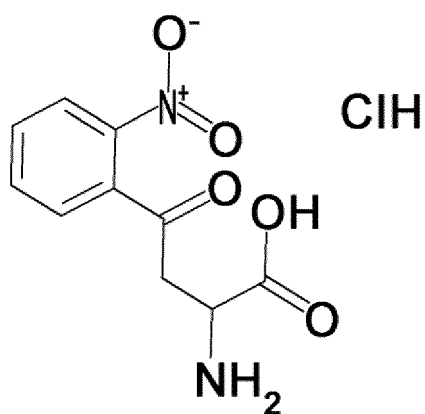
[Compound 24]
