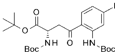
[Compound 30]
