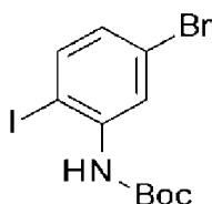
[Compound 27]
