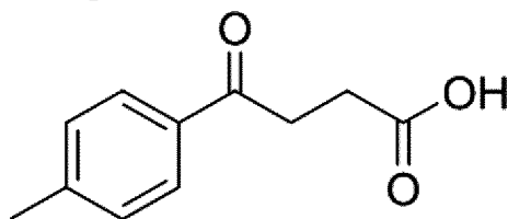
4-(4-Methylphenyl)-4-oxobutyric acid
