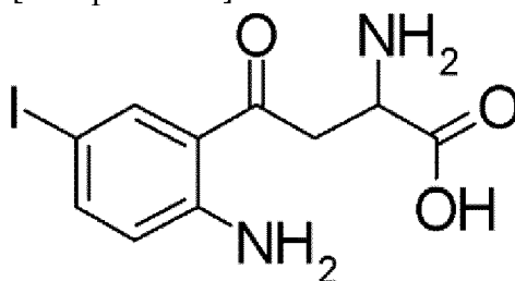
[Compound 25]
