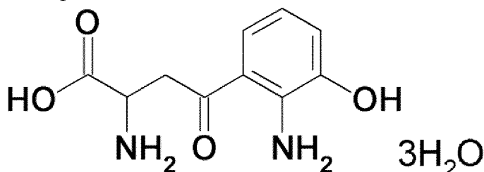
3-Hydroxy-DL-kynurenine
