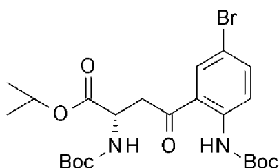
[Compound 37]
