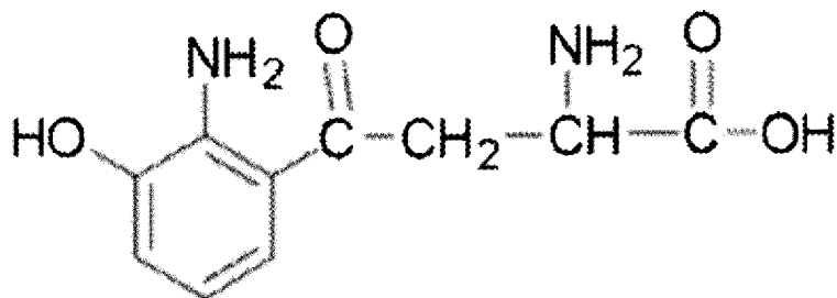
[Compound 3]
