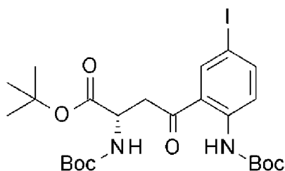
[Compound 38]
