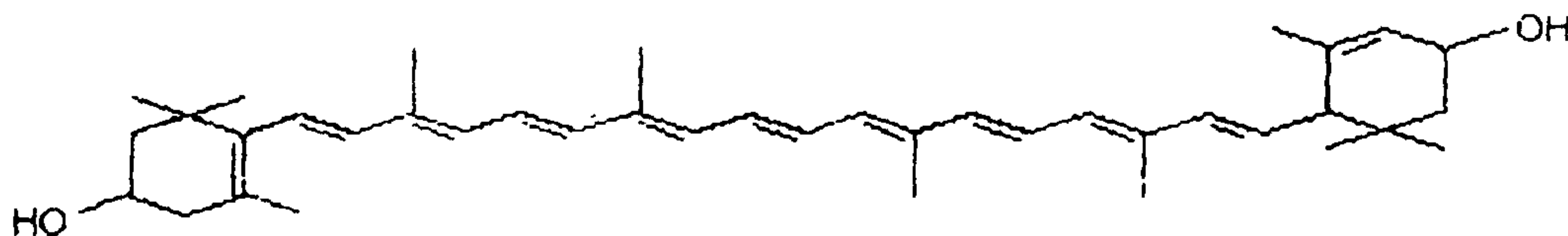
LUTEIN MOLECULE
