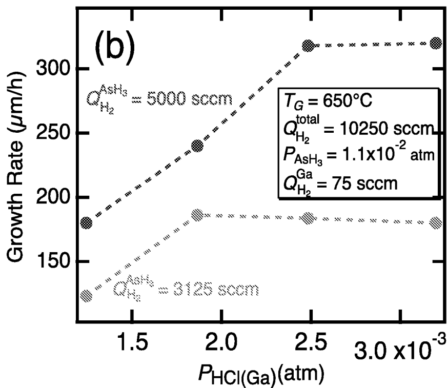
FIGs. 6(a) and 6(b)
