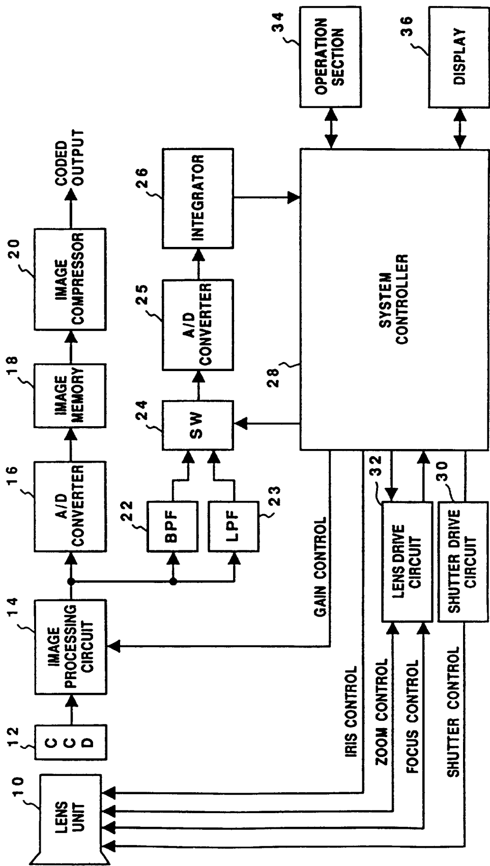
FIG. 21 PRIOR ART
