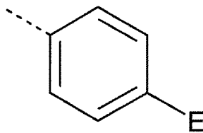
Formel (III)
