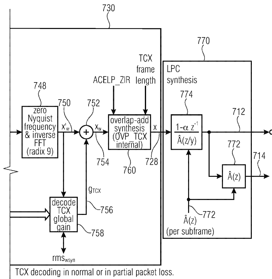
Block diagram of the TCX decoder
