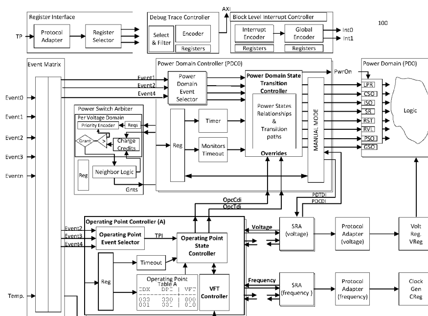
Figure 1: power domain controller &amp; operating point controller communication
