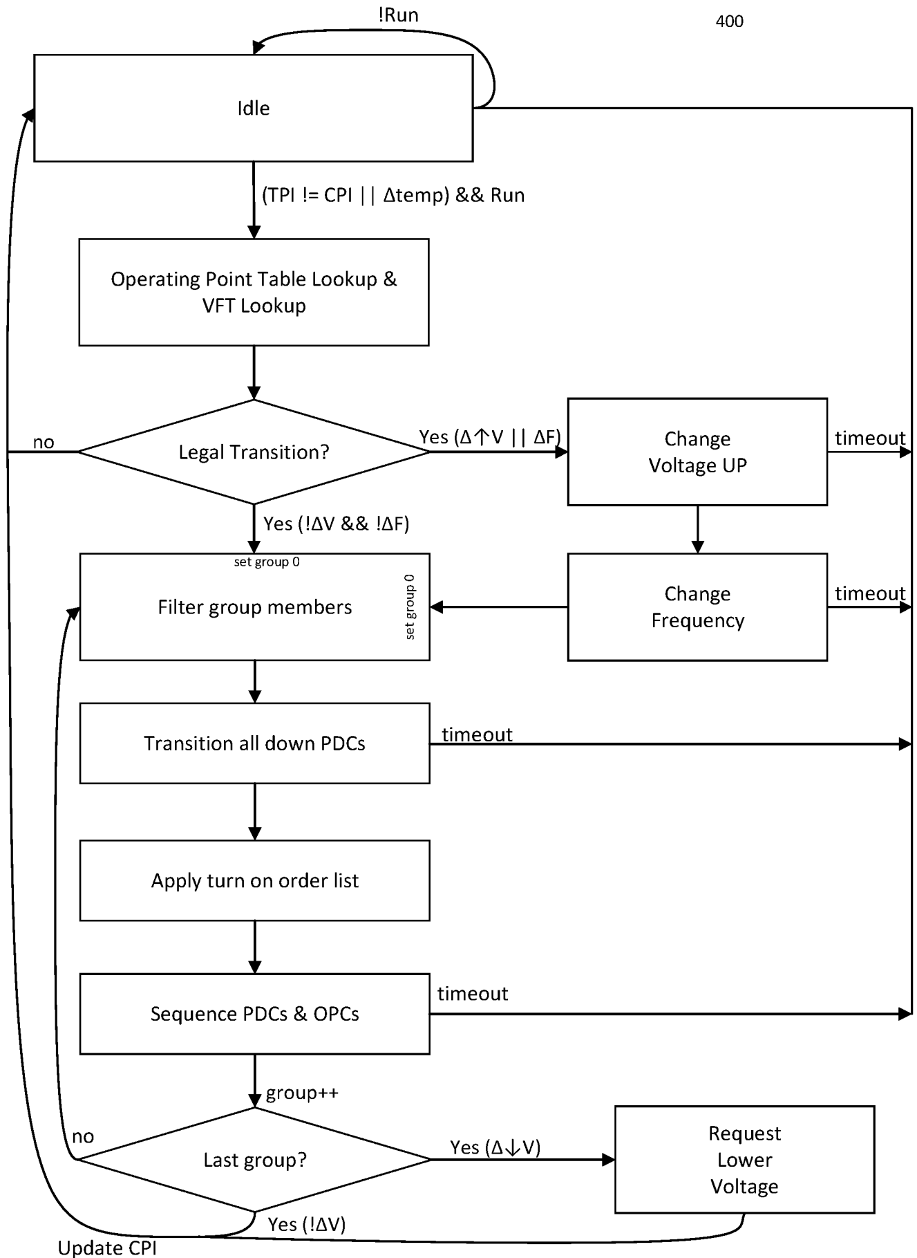
Figure 4: OPC State Machine
