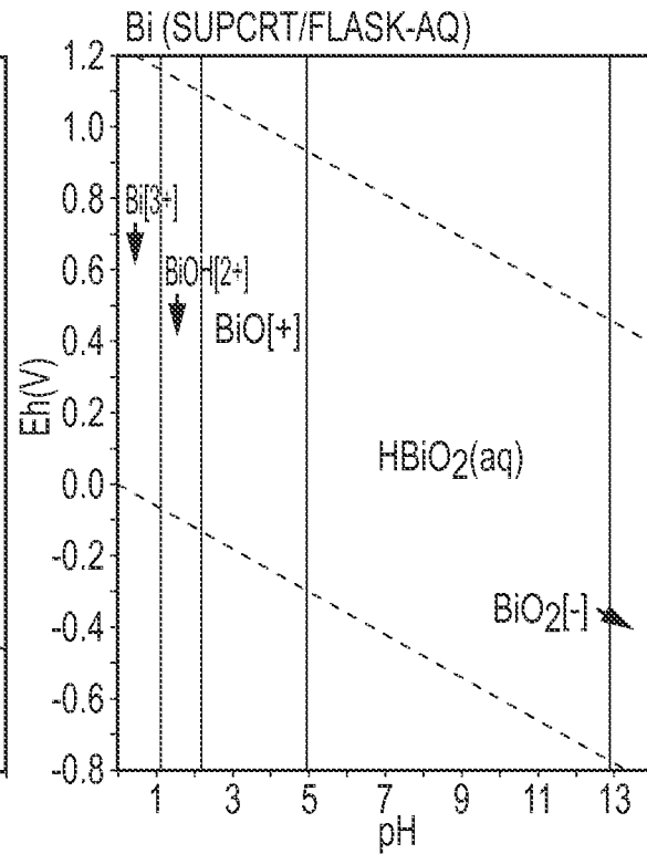
FIG.40B PRIOR ART
