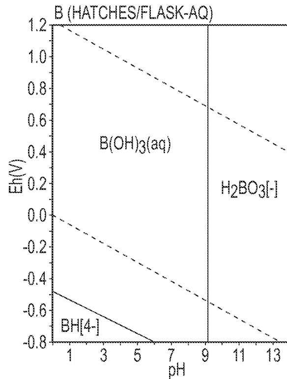
FIG.2E PRIOR ART
