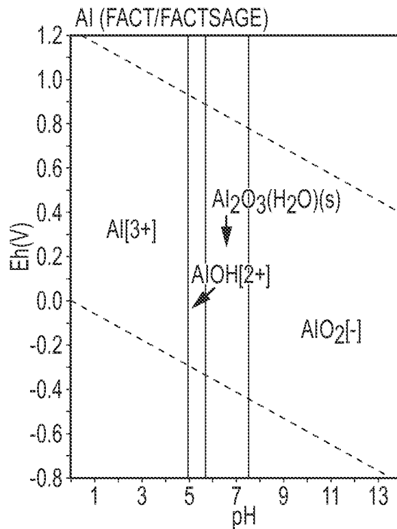
PRIOR ART FIG.3A
