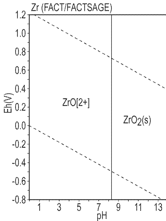
PRIOR ART FIG.16A
