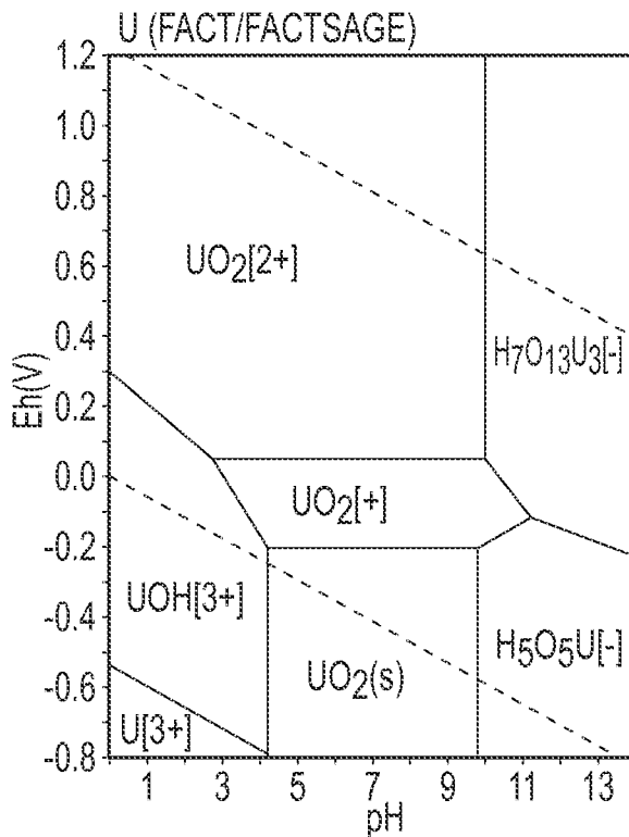
PRIOR ART FIG.45A
