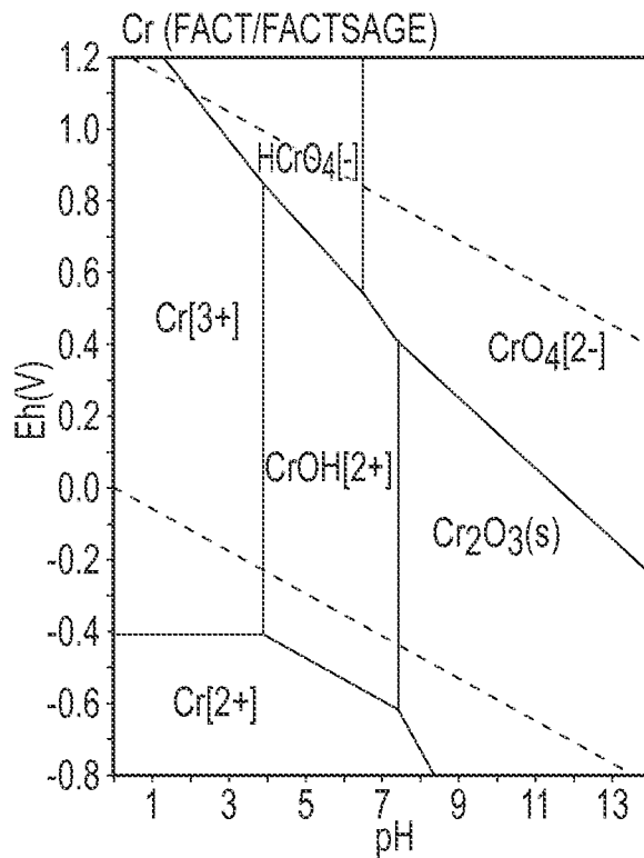
FIG.6A PRIOR ART
