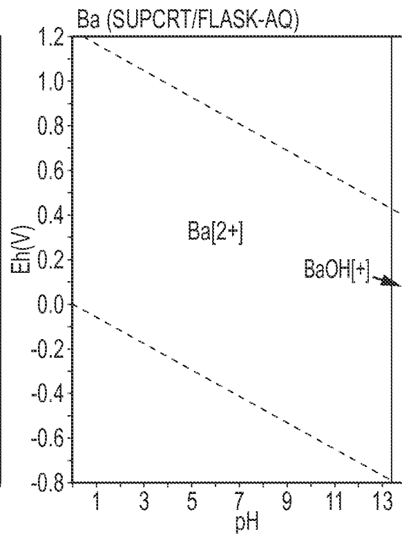
FIG.66B PRIOR ART
