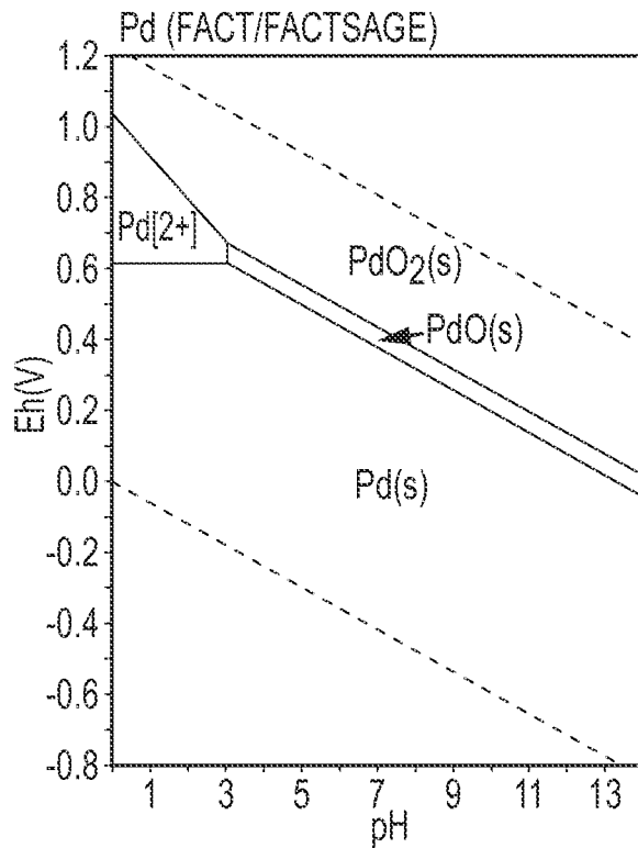
PRIOR ART FIG.22A
