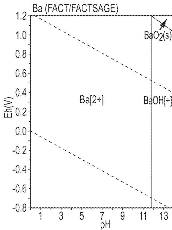
FIG.66A PRIOR ART
