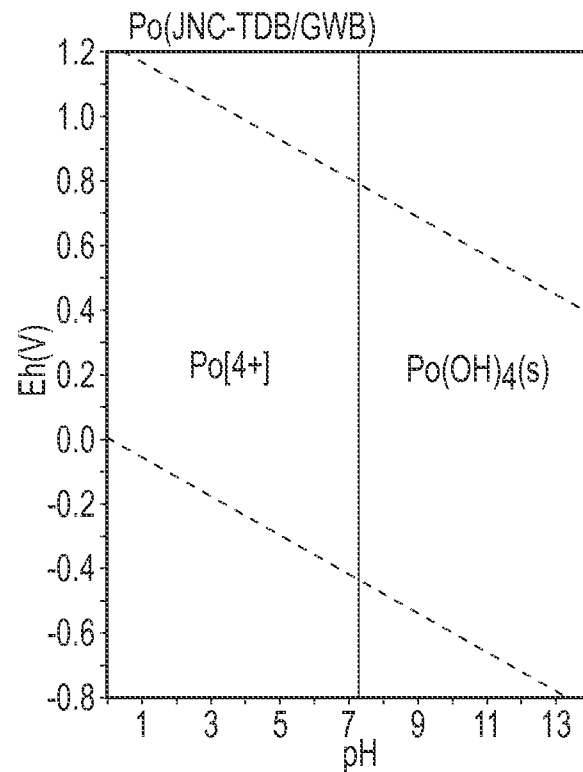
FIG.41B PRIOR ART
