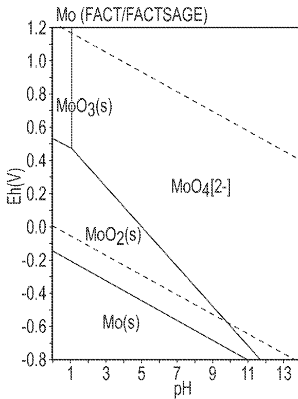
FIG.18A PRIOR ART
