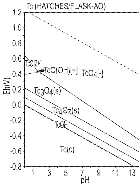
PRIOR ART FIG.19D
