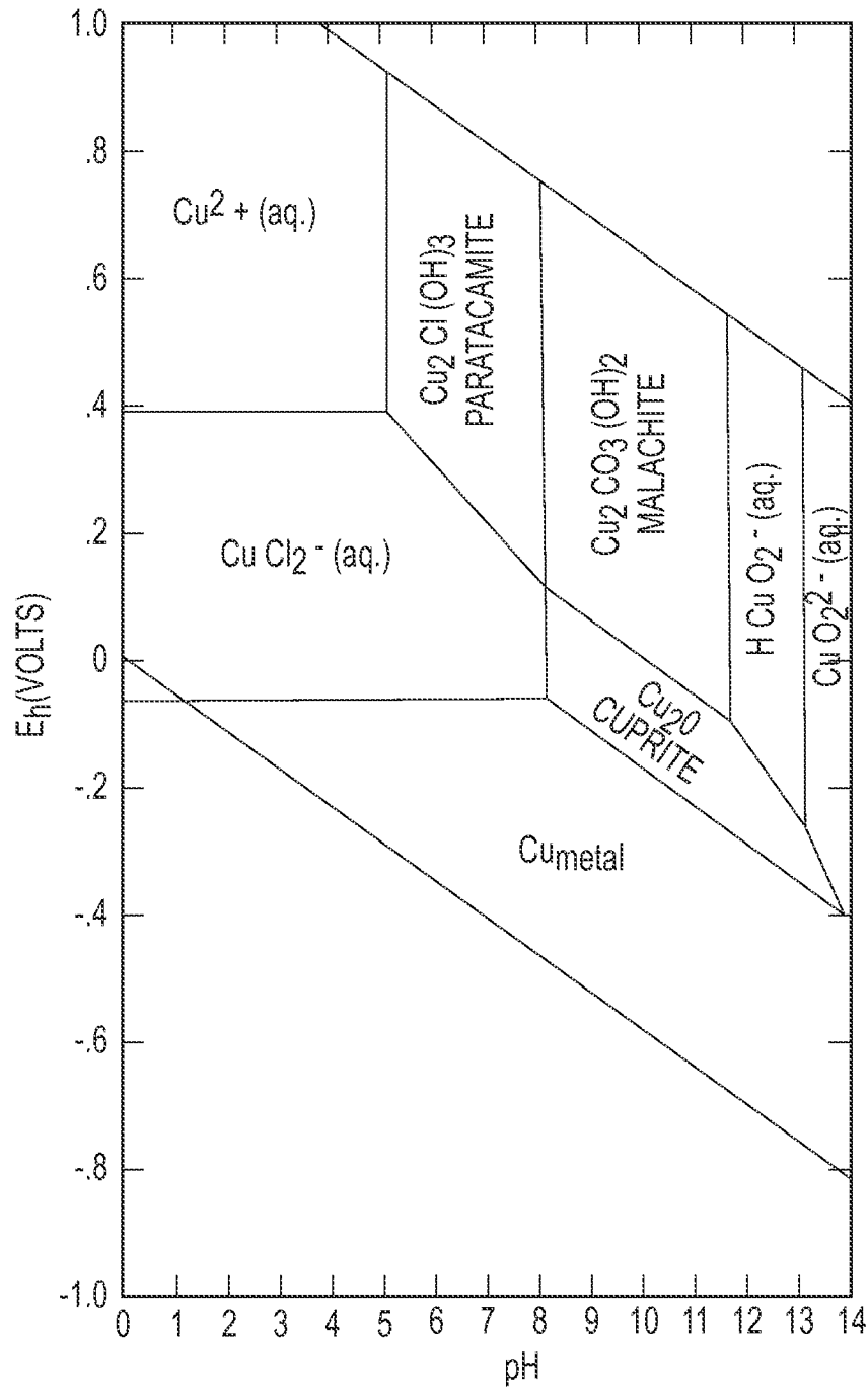
FIG.11E PRIOR ART
