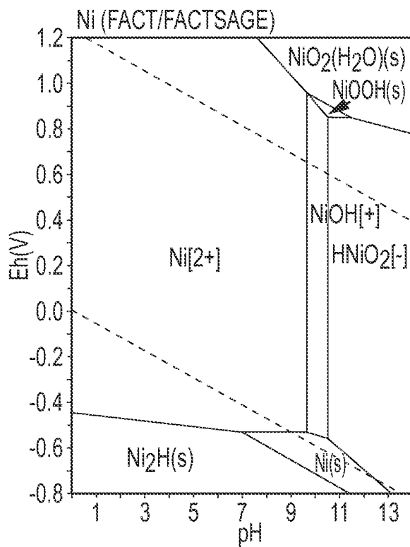
PRIOR ART FIG.10A
