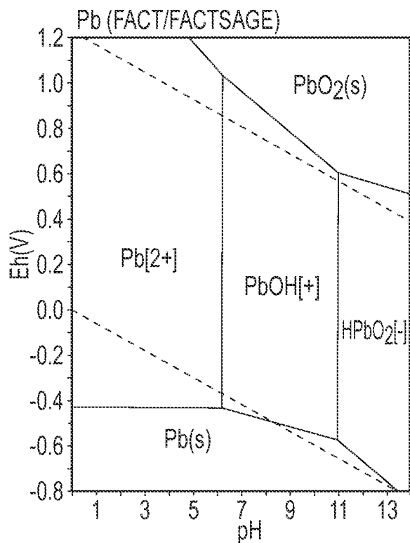
PRIOR ART FIG.38A
