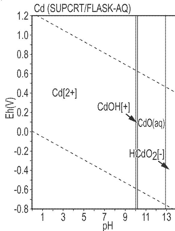
FIG.24B PRIOR ART
