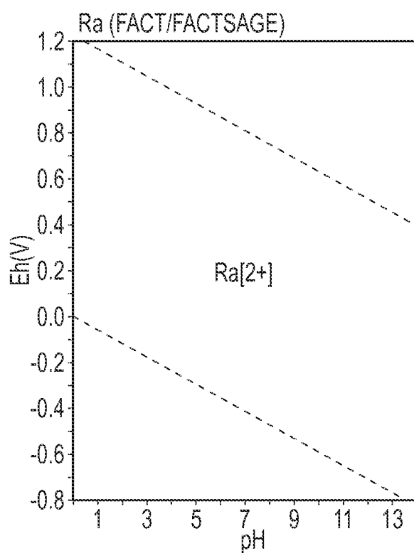
FIG.67A PRIOR ART
