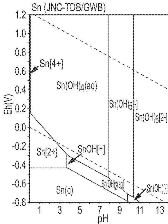
PRIOR ART FIG.26D
