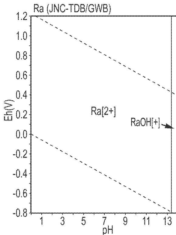
FIG.67D PRIOR ART
