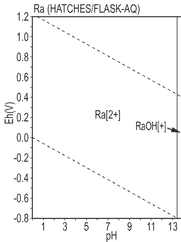
FIG.67E PRIOR ART
