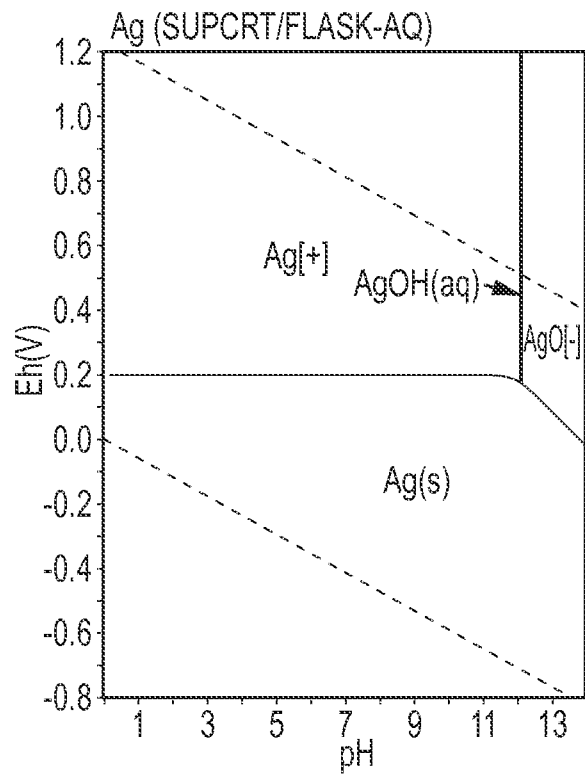
FIG. 23B PRIOR ART
