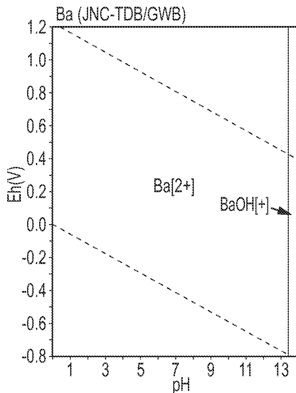
FIG.66D PRIOR ART
