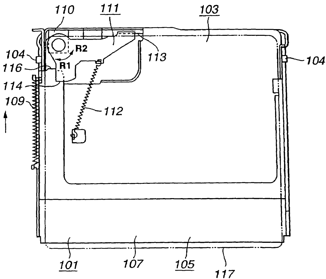
FIG. 4 (PRIOR ART)
