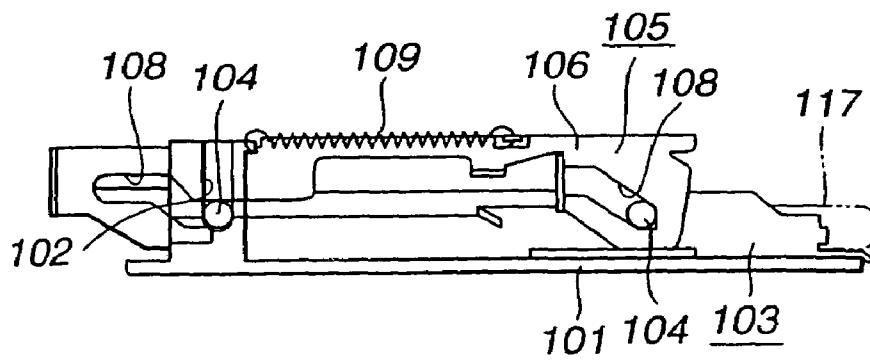
FIG. 5 (PRIOR ART)
