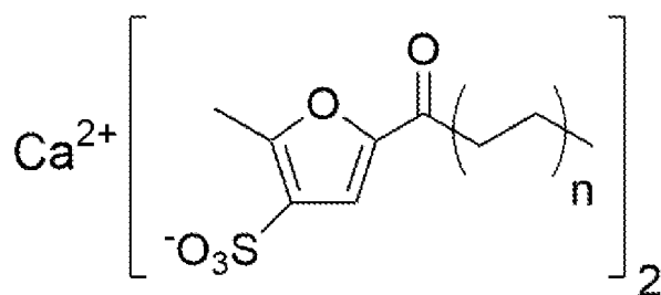
Structure A of General Structure 1
