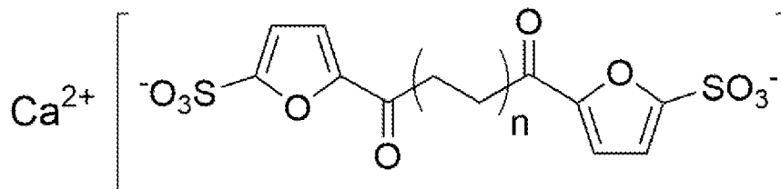
Structure C of General Structure 1
