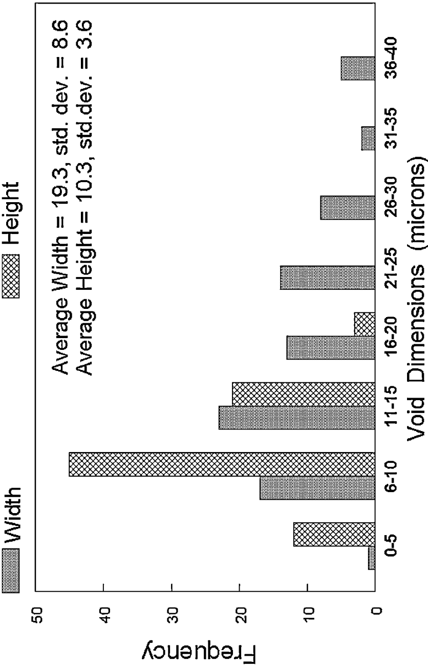
Fig. 17 Distribution of Void Dimensions
