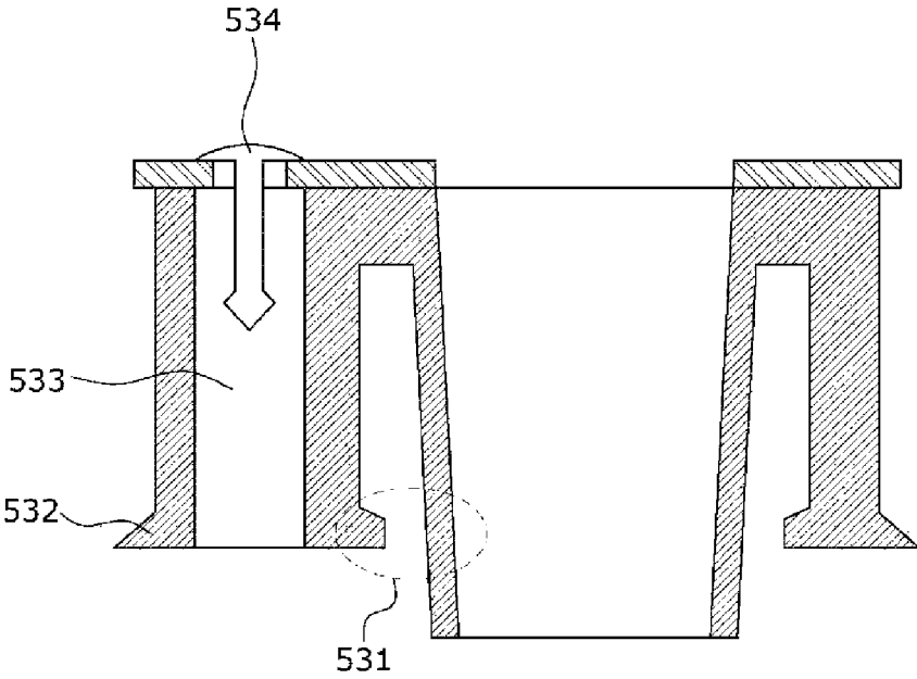
CROSS-SECTIONAL DIAGRAM TAKEN ALONG THE LINE A-A
